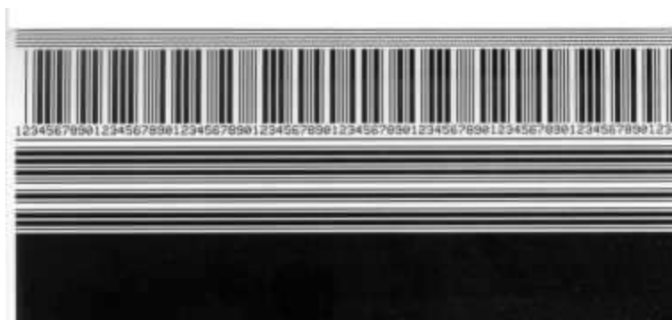
Typical Zebra Printer Test Label (Properly Balanced)
