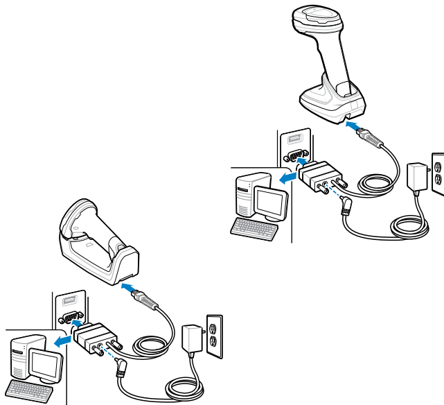
Figure 4 RSR Connection
