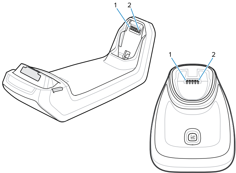
Figure 6 Cradle Pin-Outs
