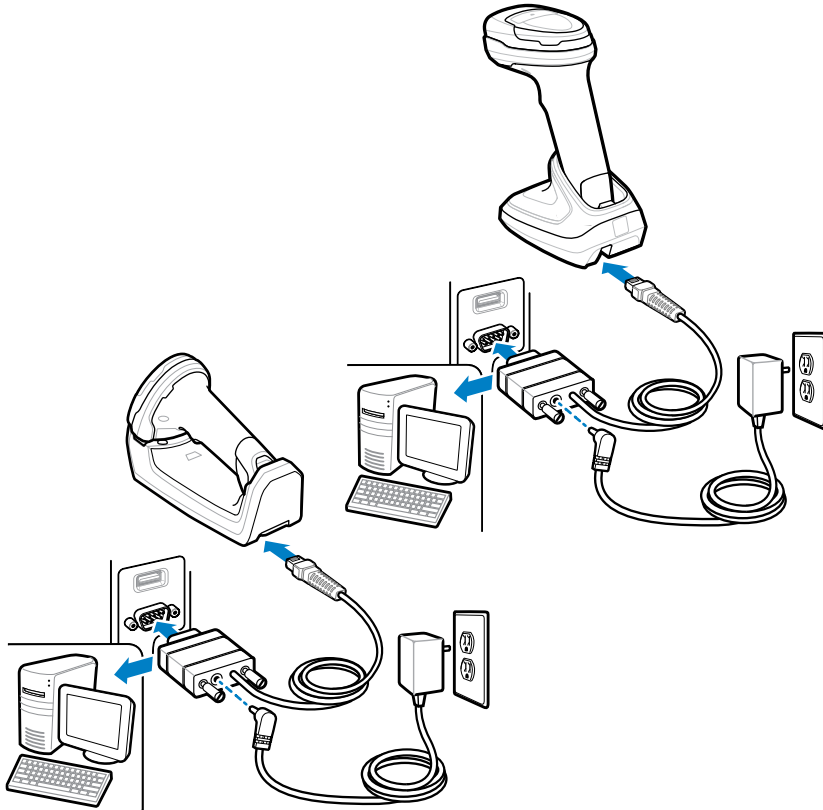
Figure 8 RS-232 Connection
