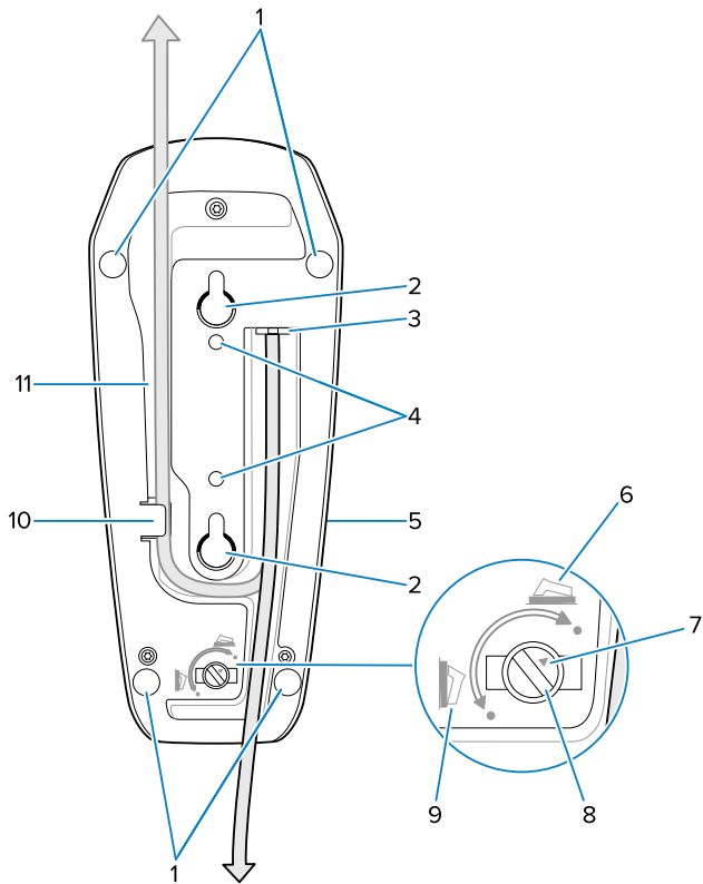
Figure 3 Bottom View
