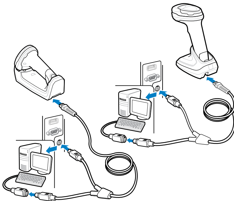
Figure 10 Keyboard Wedge Connection
