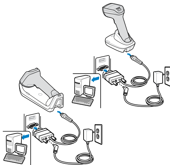
Cordless DS8288/DS8288R RS-232 Connection
