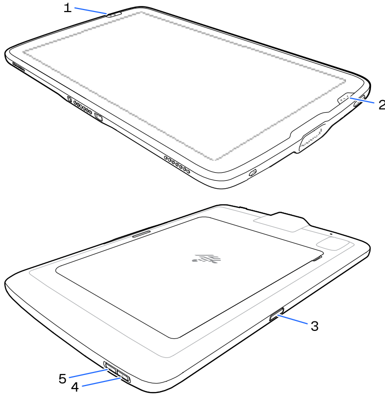
Figure 9 Key Positions
