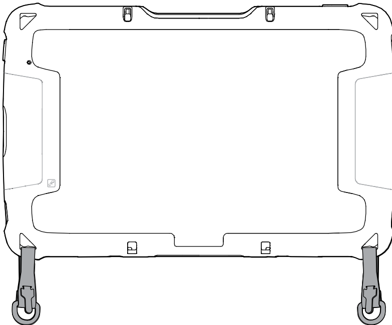
Figure 38 D-Clips - Portrait
