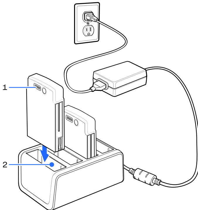
Figure 37 4-Slot PowerPack Battery Charger
