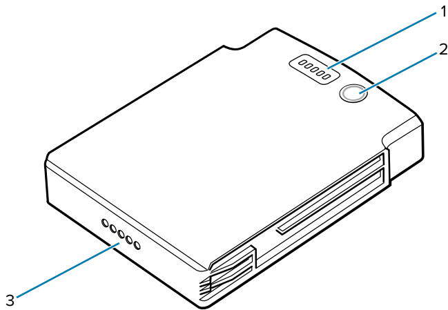
Figure 52 Power Pack
