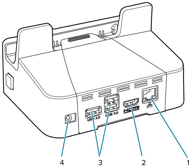
Figure 44 Rugged Communication and Charging Cradle - Rear View
