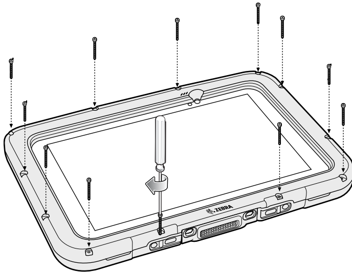
Figure 54 Secure 10 in. Rugged Frame
