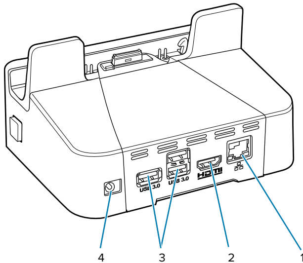
Figure 39 Communication and Charging Cradle - Rear View
