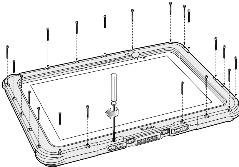
Figure 54 Secure 10 in. Rugged Frame
