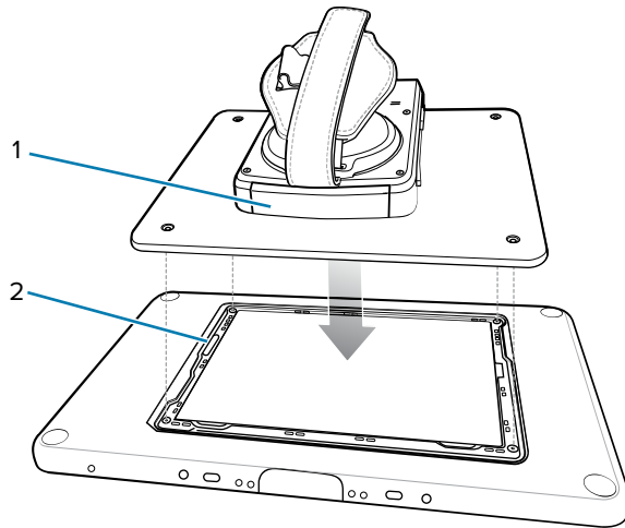
Figure 56 Align Expansion Back with 10 in. Device
