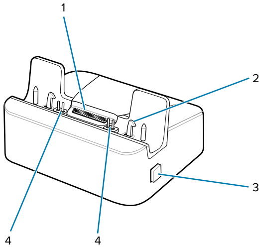
Figure 43 Rugged Communication and Charging Cradle - Front View
