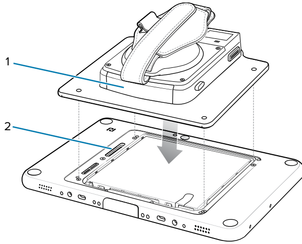
Figure 56 Align Expansion Back with 10 in. Device
