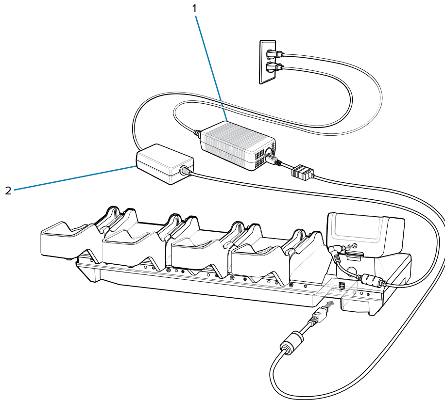
Figure 47 Power Setup with Optional Charger
