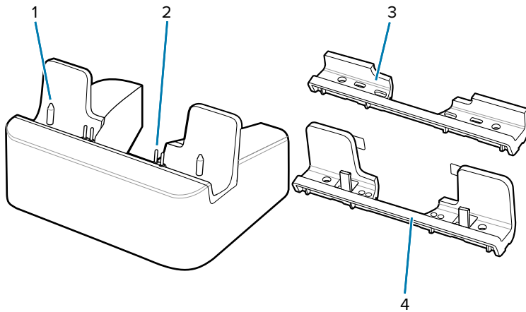
Figure 36 Charge Only Cradle - Front View
