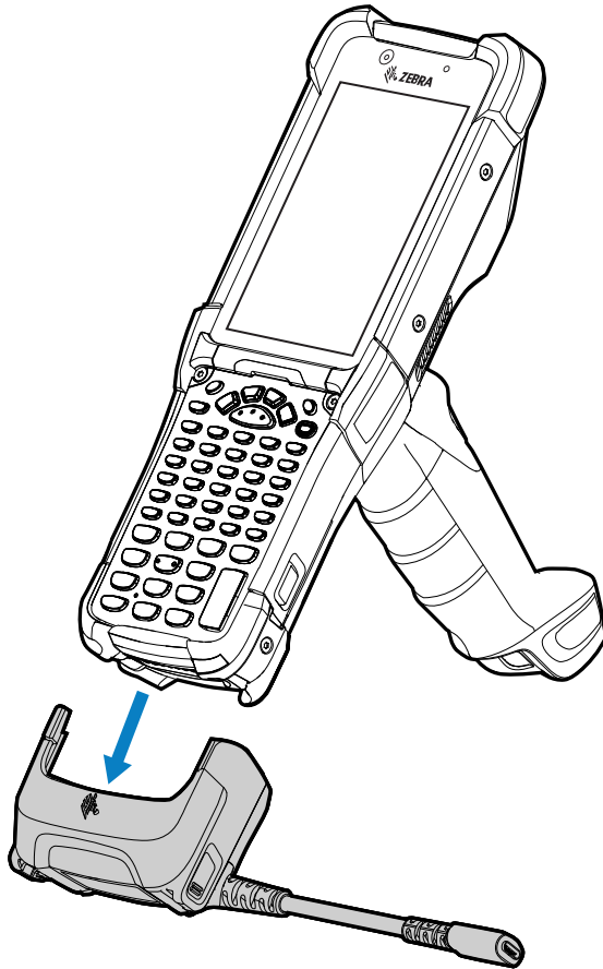
Figure 45 Connecting the USB Charge/Com Snap-on Cup
