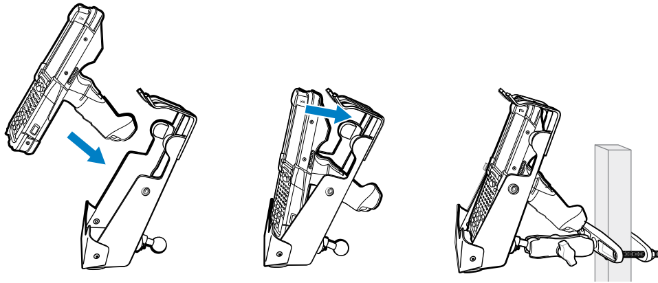
Figure 51 Insert Device into Forklift Mount Holder, Rotate and Snap (Option 2)
