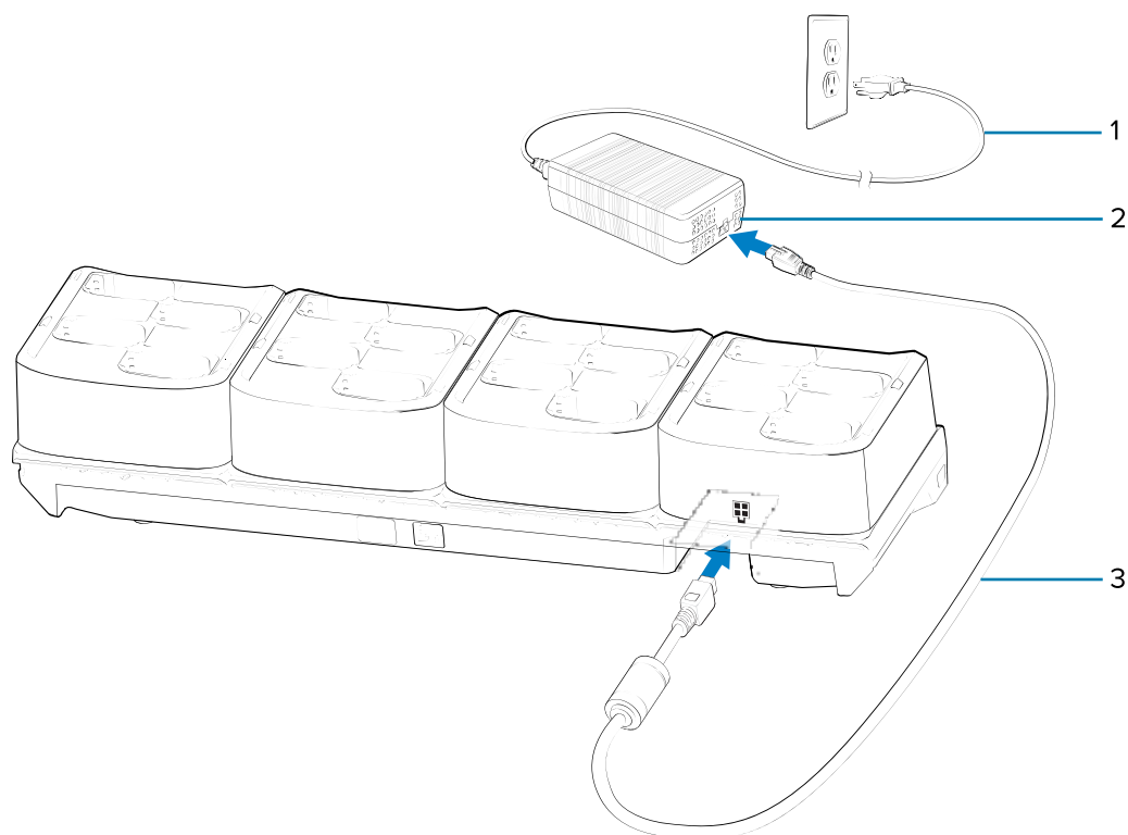
Figure 42 16-Slot Spare Battery Charger Setup
