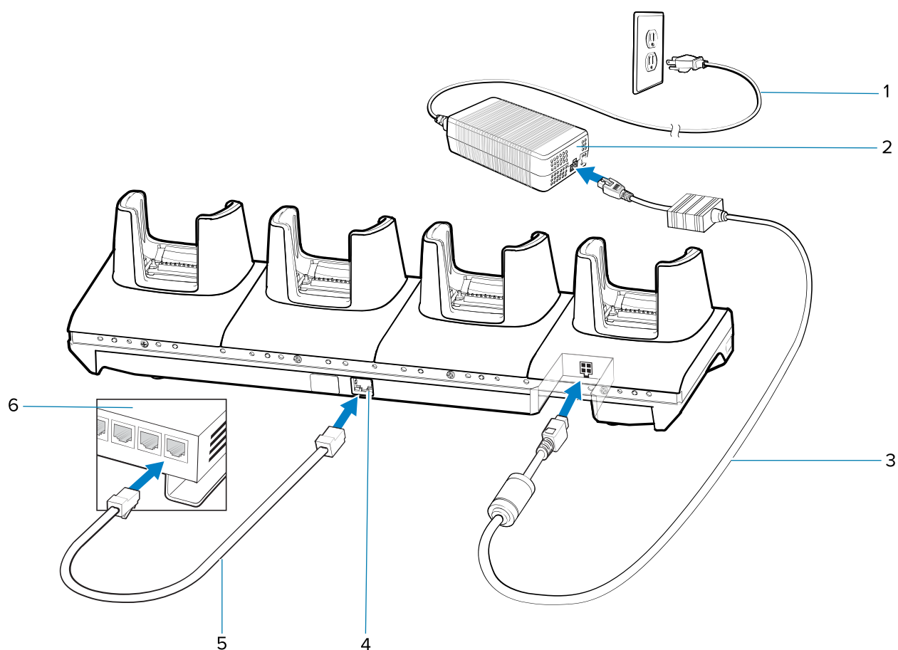
Figure 35 4-Slot Ethernet ShareCradle Setup
