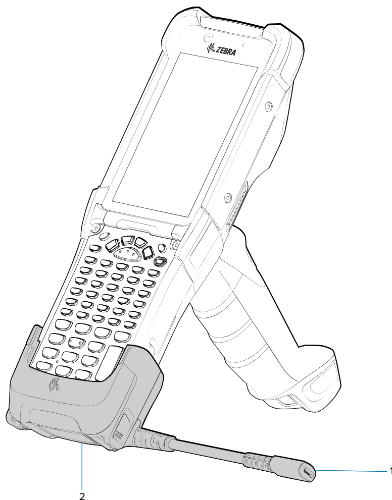
Figure 44 USB Charge/Com Snap-on Cup
