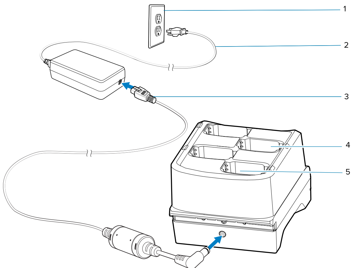
Figure 39 4-Slot Spare Battery Charger Setup
