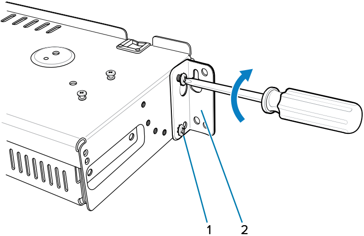
Figure 52 Flange Horizontal Position (5-Slot Cradles)
