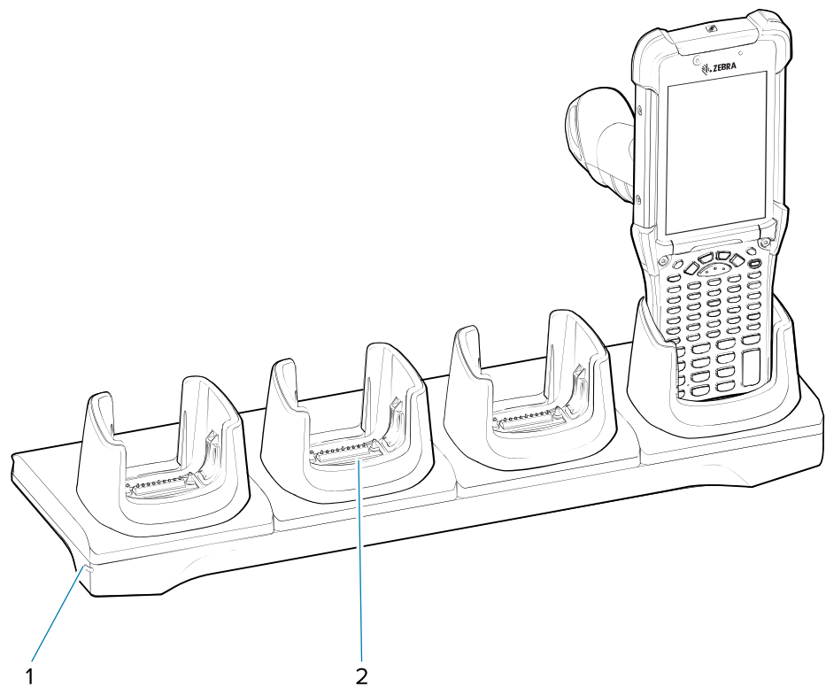
Figure 33 4-Slot Charge Only ShareCradle
