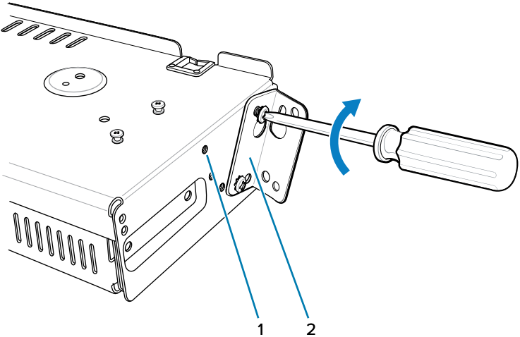
Figure 53 Flange 25° Position (4-Slot Battery Chargers)
