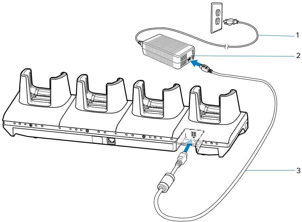
Figure 32 4-Slot Charge Only ShareCradle Setup
