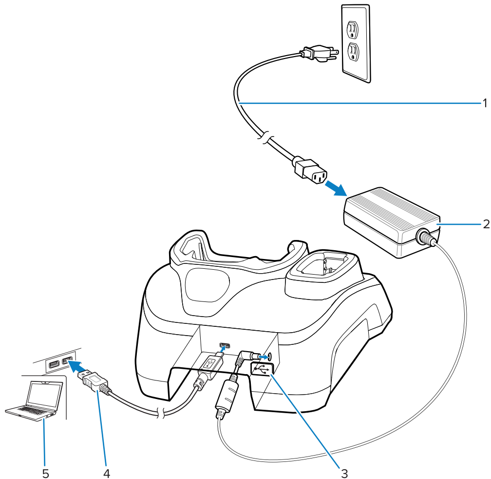
Figure 29 1-Slot USB Charge Cradle with Spare Battery Charger Setup
