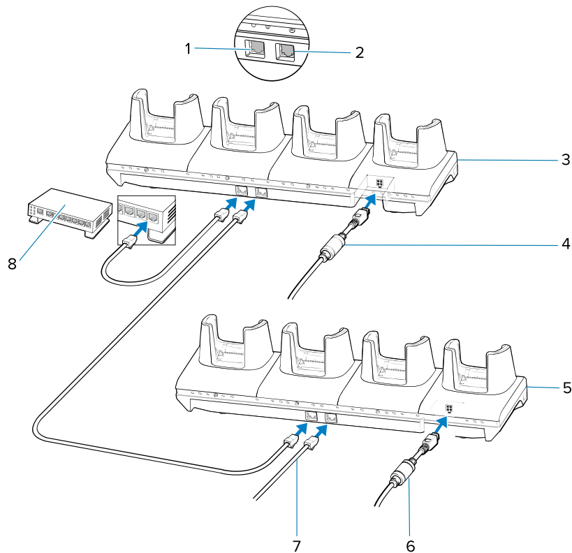
Figure 37 Daisy-chaining 4-Slot Ethernet ShareCradles
