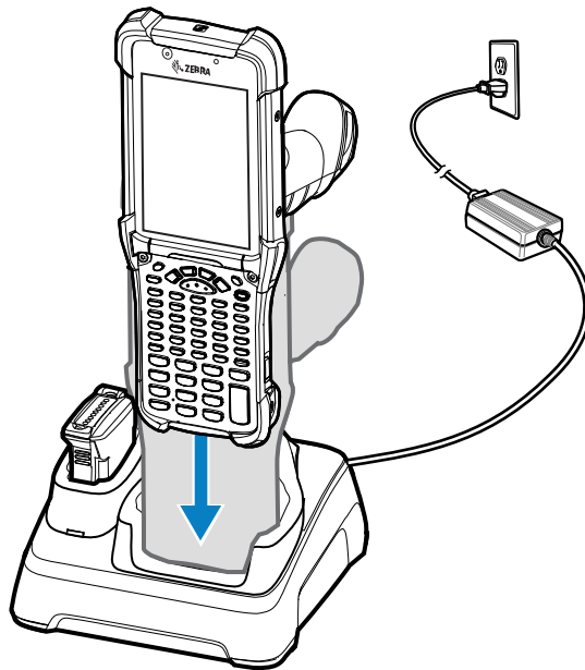
Figure 30 1-Slot USB Charge Cradle with Spare Battery Charger
