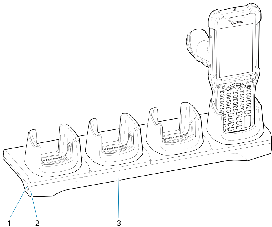
Figure 6 4-Slot Ethernet ShareCradle
