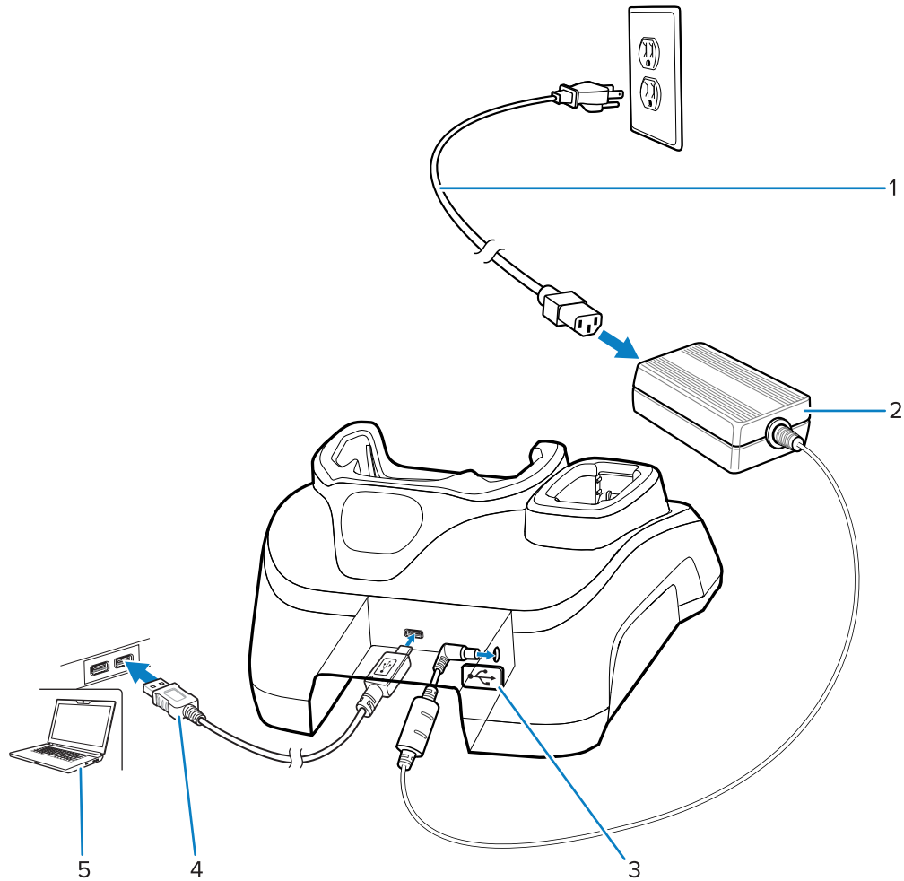
Figure 15 1-Slot USB Charge Cradle with Spare Battery Charger Setup
