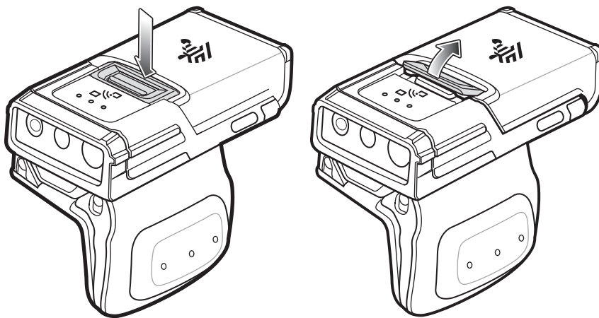
Figure 4 Release Battery
