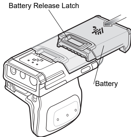
Figure 3 Install the Battery
