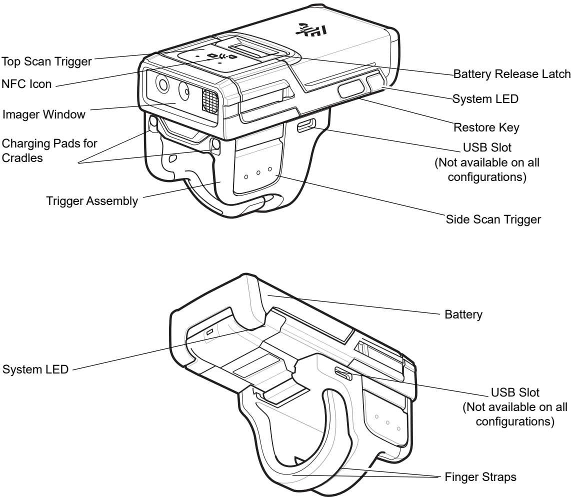
Figure 2 RS5100 Double Trigger Configuration Features
