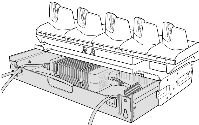
Figure 146 Slide Top Tray onto Bottom Tray
