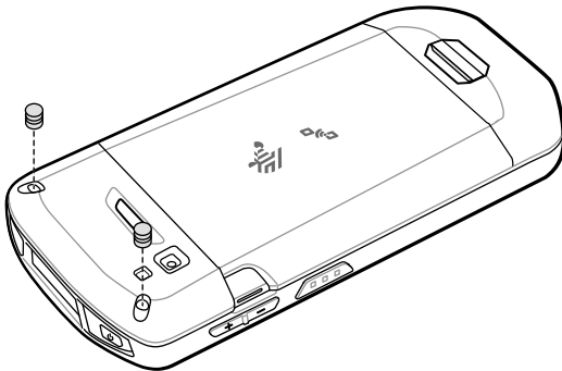
Figure 111 Remove Plugs
