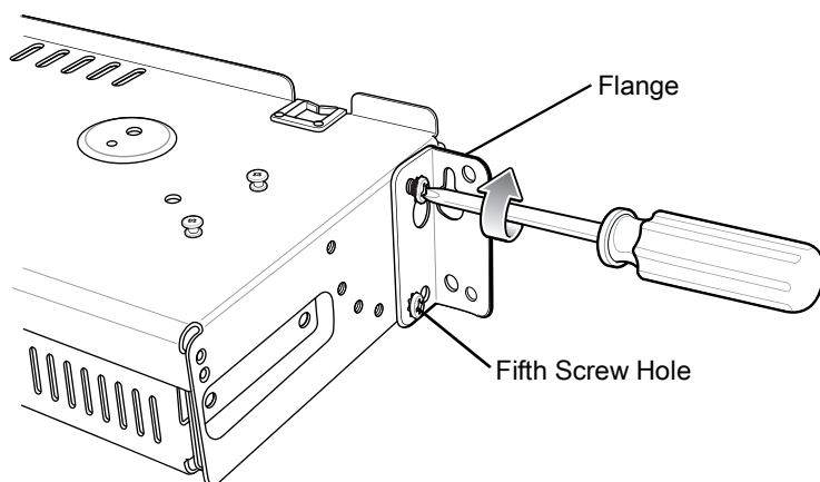
Figure 156 Flange 25° Position (4-Slot Battery Chargers)
