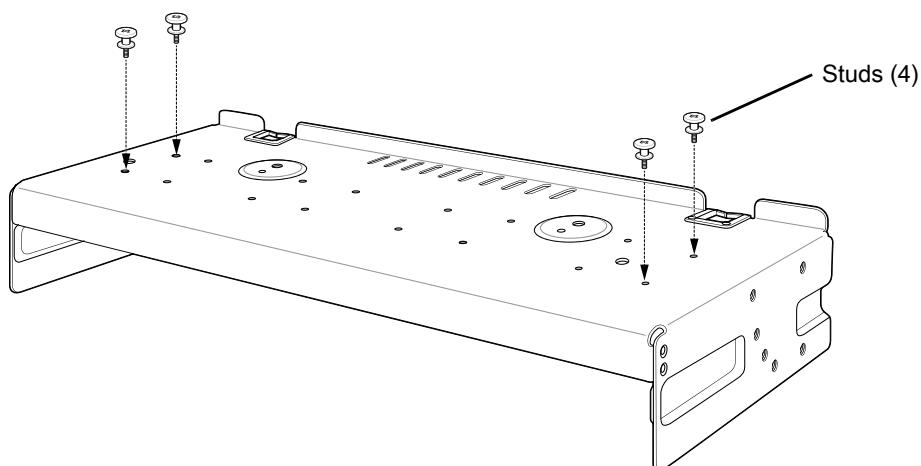
Figure 143 Install Studs
