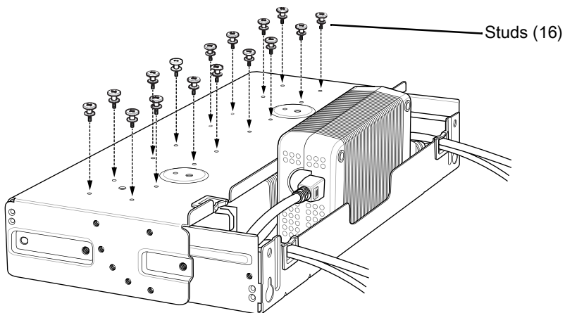
Figure 151 Install Studs
