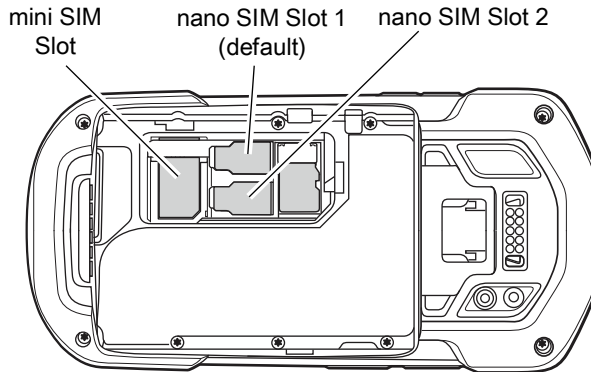
Figure 1 TC75x SIM Slot Locations
