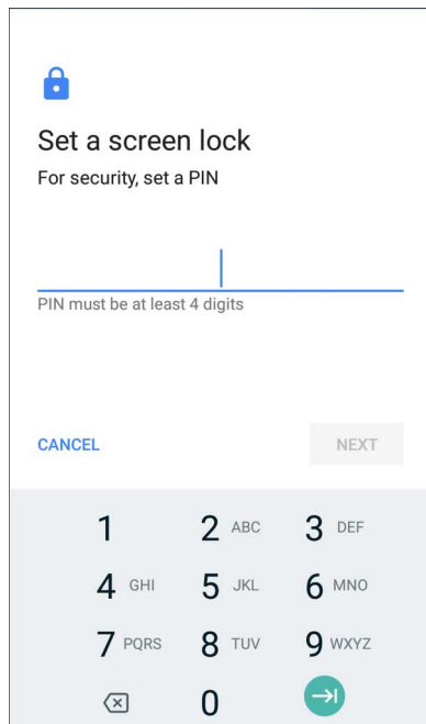
Figure 95 PIN Screen
