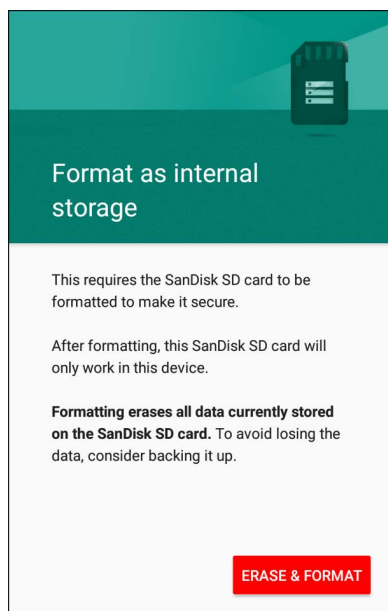
Figure 147 Format Screen
