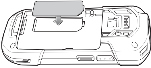
Figure 22 Replace Access Door
