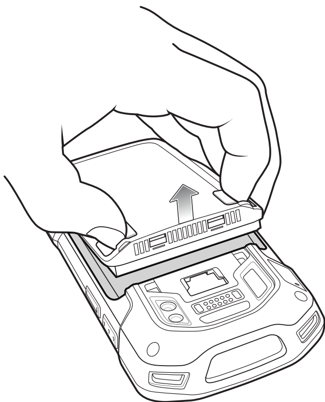
Figure 81 Lift the Battery
