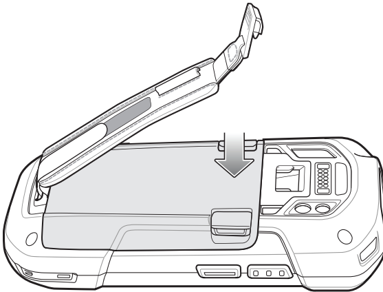
Figure 84 Press Down on Battery
