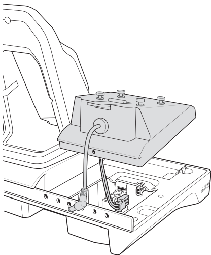
Figure 63 Connect Adapter Power Cable
