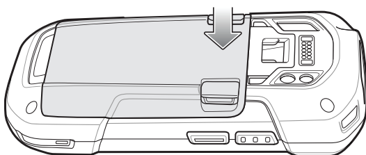
Figure 12 Press Down on Battery
