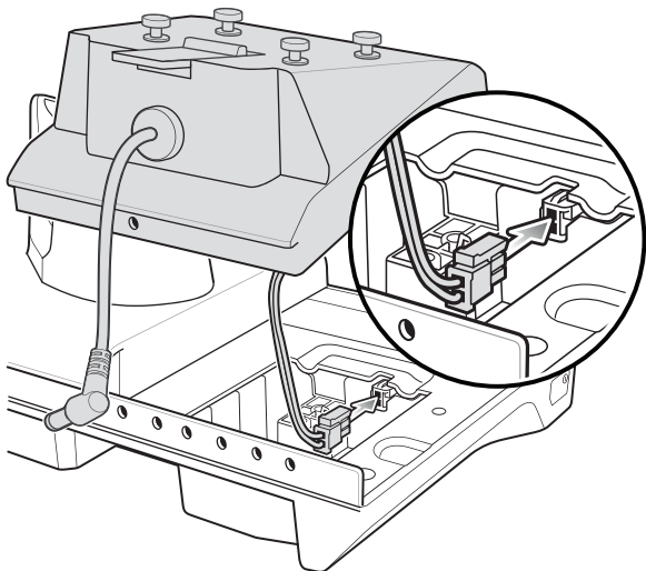
Figure 46 Connect Adapter Power Cable
