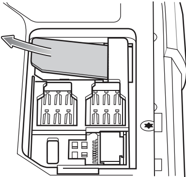
Figure 19 Remove Nano SIM Card
