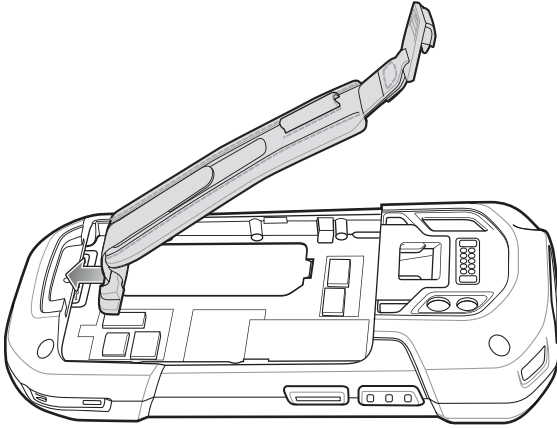
Figure 82 Insert Hand Strap
