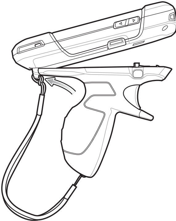
Figure 75 Connect Device to Trigger Handle
