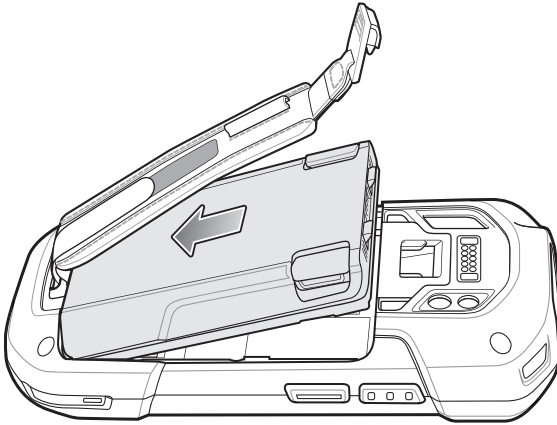
Figure 83 Insert Bottom of Battery into Battery Compartment
