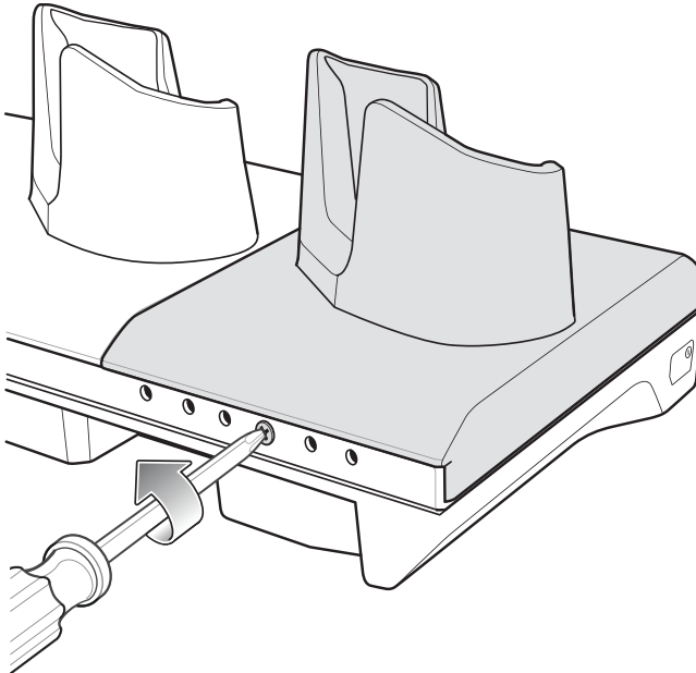
Figure 43 Remove Screw
