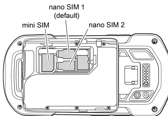
Figure 86 TC75x SIM Slot
