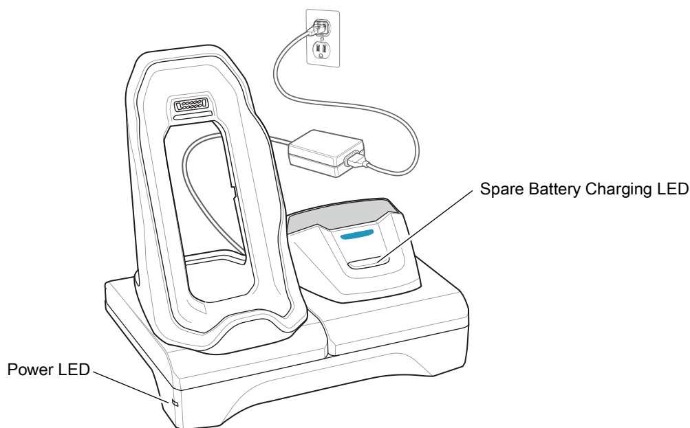
Figure 30 2-Slot USB/Ethernet Cradle
