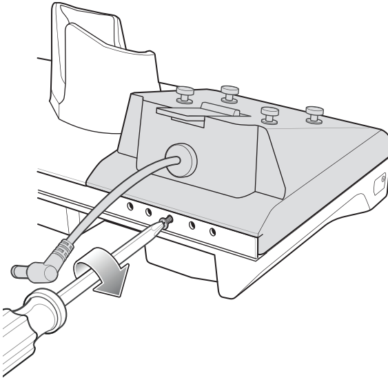
Figure 48 Secure adapter to Cradle
