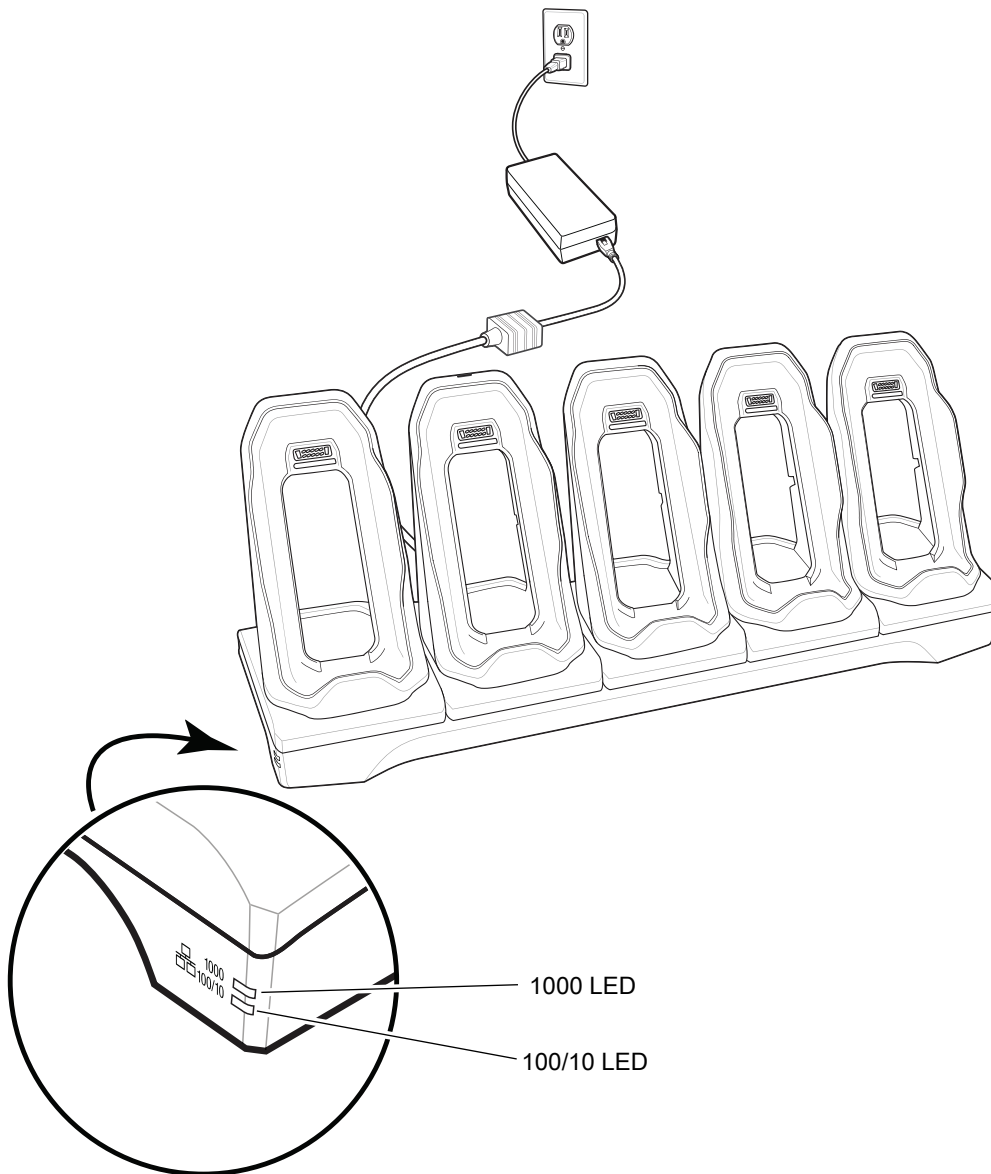
Figure 52 5-Slot Ethernet Cradle
