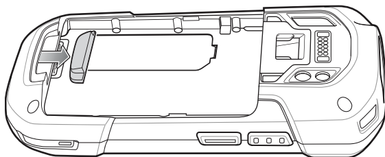
Figure 73 Remove Hand Strap Plate
