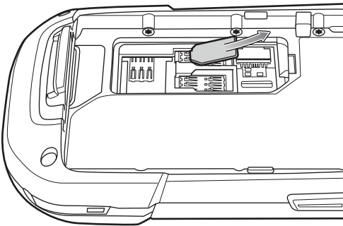
Figure 19 Remove Nano SIM Card
