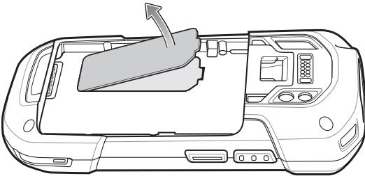
Figure 17 Remove Access Door
