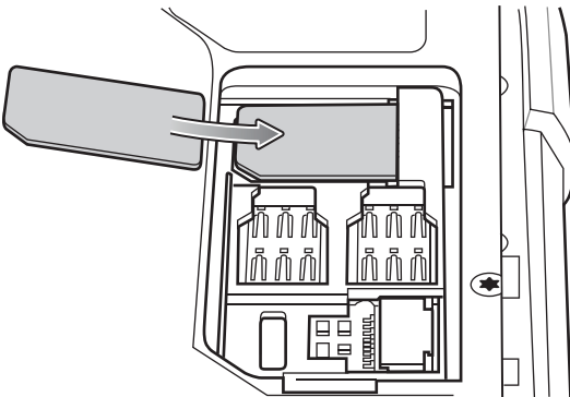
Figure 21 Insert Nano SIM Card
