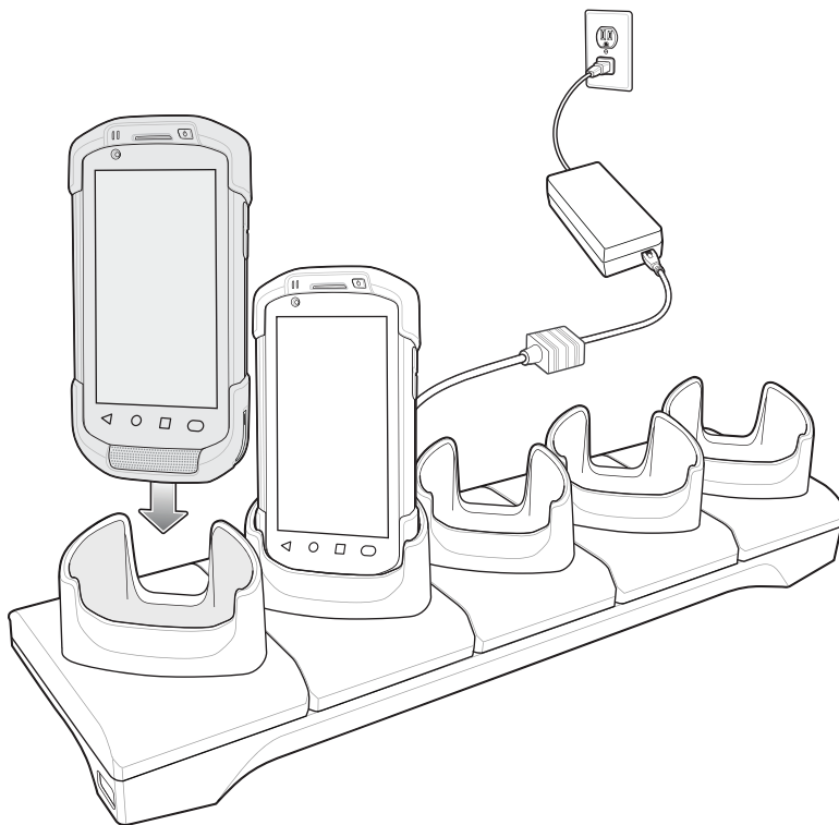
Figure 41 5-Slot Charge Only Cradle with Four Slot Battery Charger
