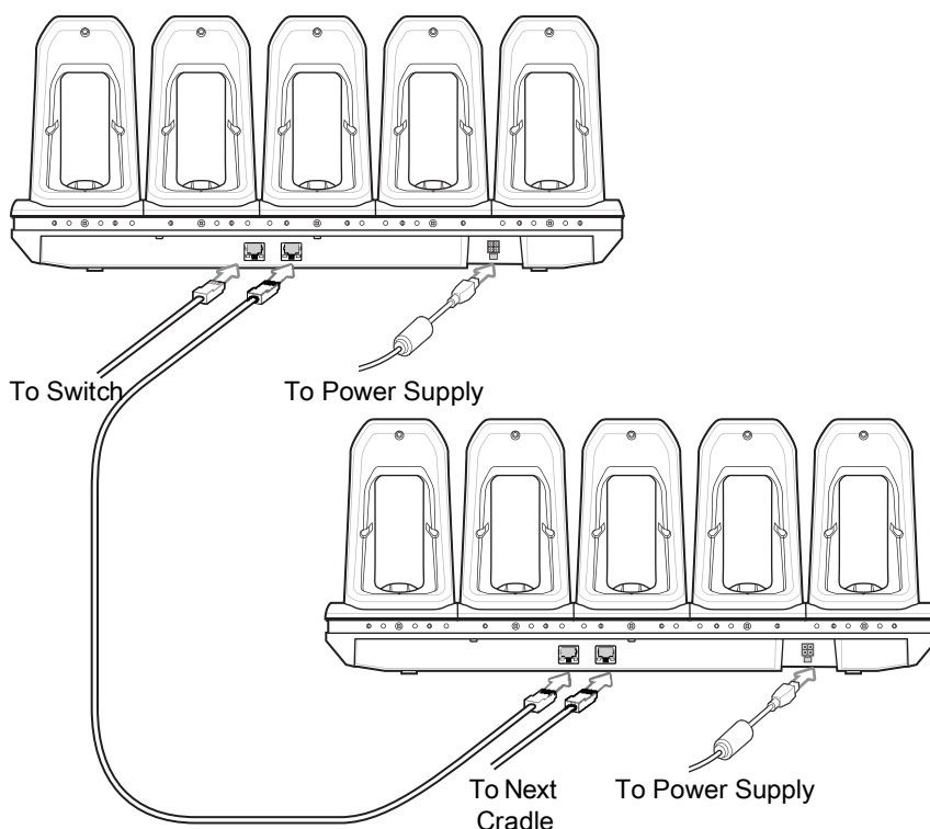
Figure 54 Daisy-chaining 5-Slot Ethernet Cradles
