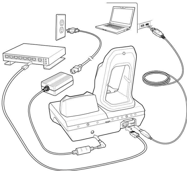
Figure 31 2-Slot USB/Ethernet Cradle
