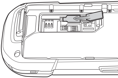
Figure 3 Mini SIM Card Installation
