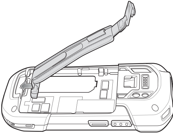
Figure 7 Insert Hand Strap
