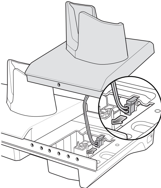
Figure 45 Disconnect Cup Power Cable
