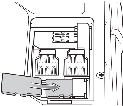
Figure 5 Insert microSD Card in Holder
