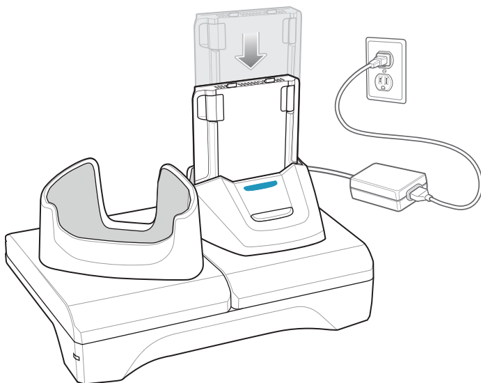
Figure 29 Spare Battery Charging
