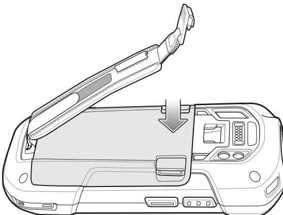
Figure 9 Press Down on Battery
