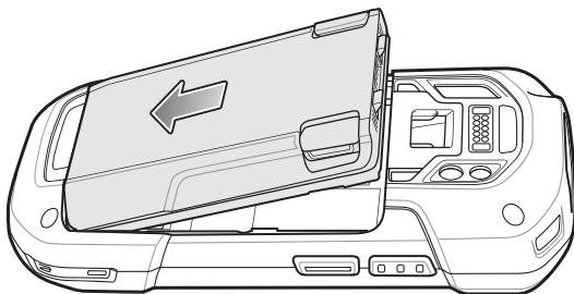
Figure 11 Insert Bottom of Battery into Battery Compartment
