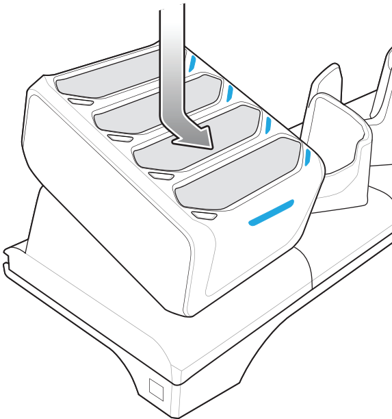
Figure 49 Install Four Slot Battery Charger
