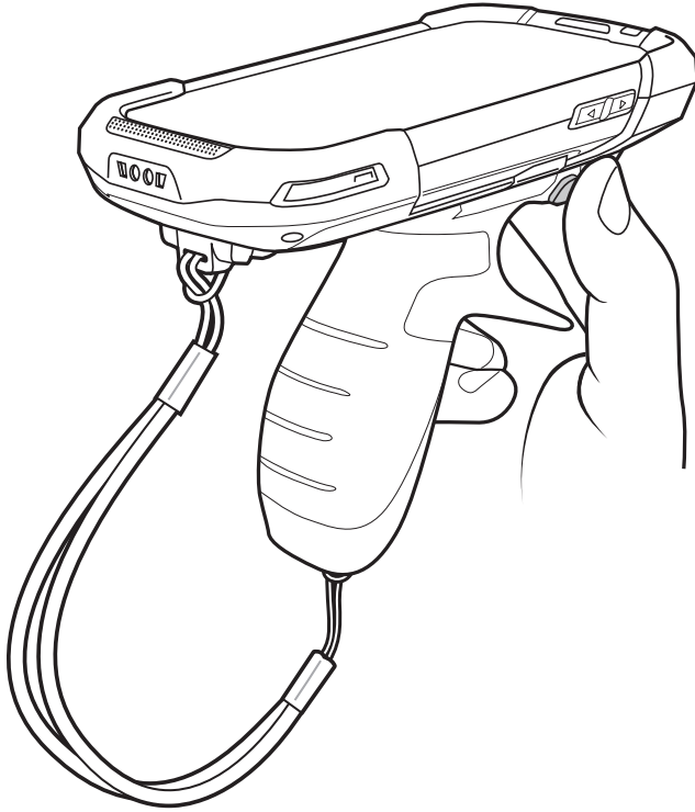
Figure 77 Press Release Latches
