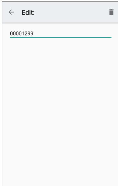
Figure 131 Formatted Data
