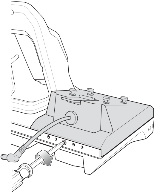
Figure 65 Secure adapter to Cradle
