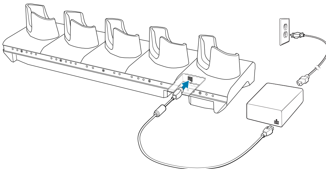
Figure 35 5-Slot Ethernet Cradle
