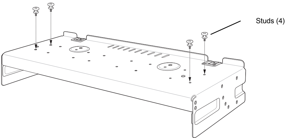
Figure 45 Install Studs
