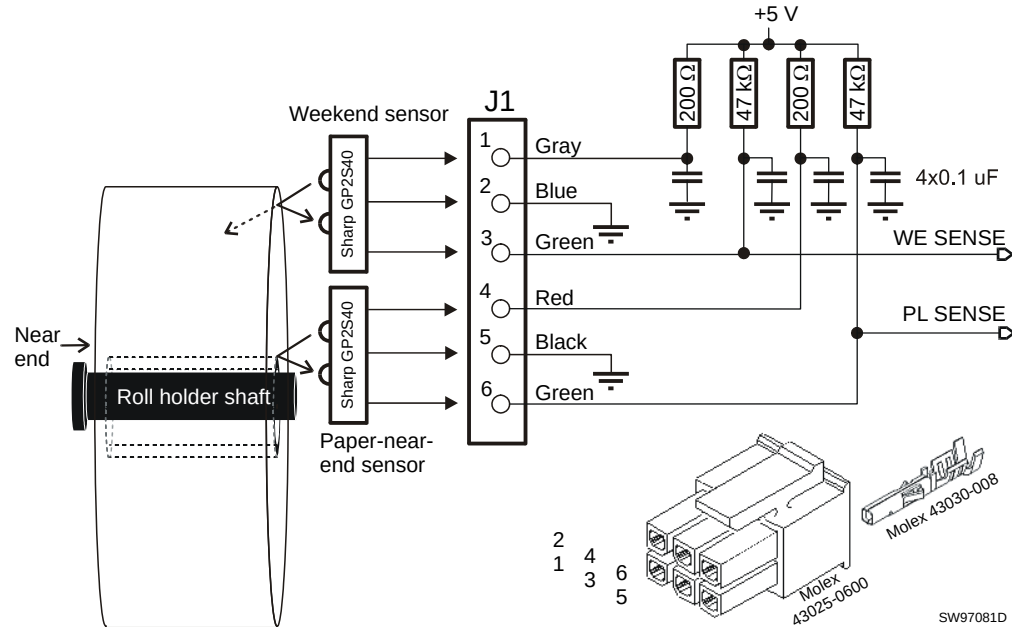
Figure 11 • Paper-near-end Sensor Connection
