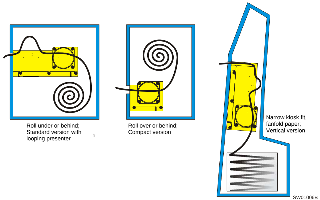
Figure 5 • Installation Options
