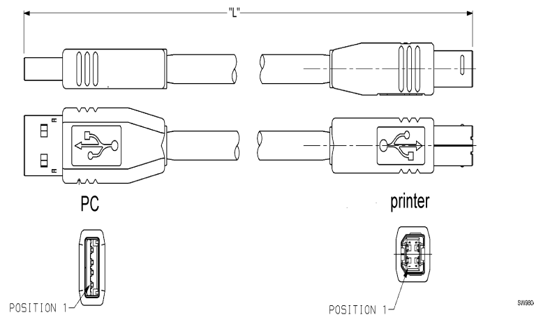
Figure 8 • USB Cable with Type A and Type B Connectors
