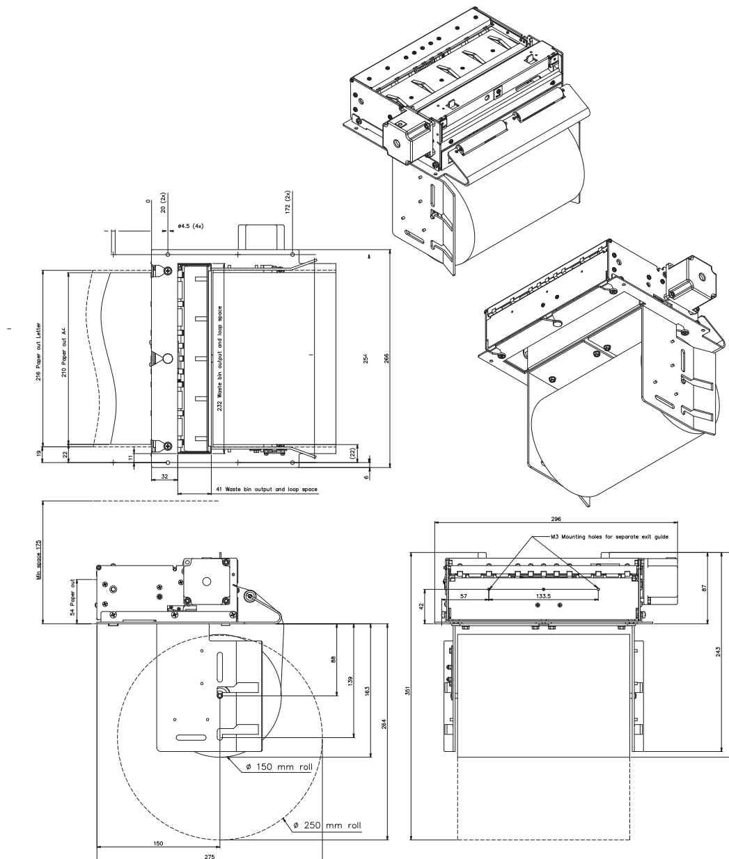
Figure 28 • Measurements Drawing, Printer 01744-xxx with Roll Holder for 150 or 250mm Roll Under Printer
