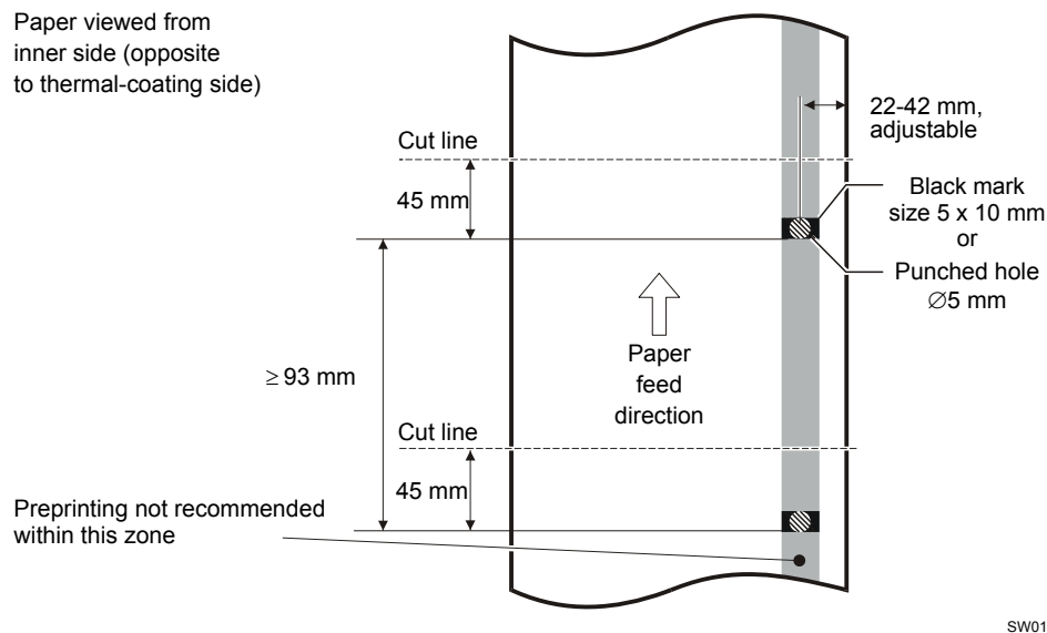
Figure 20 • Recommended Black Mark Size and Position
