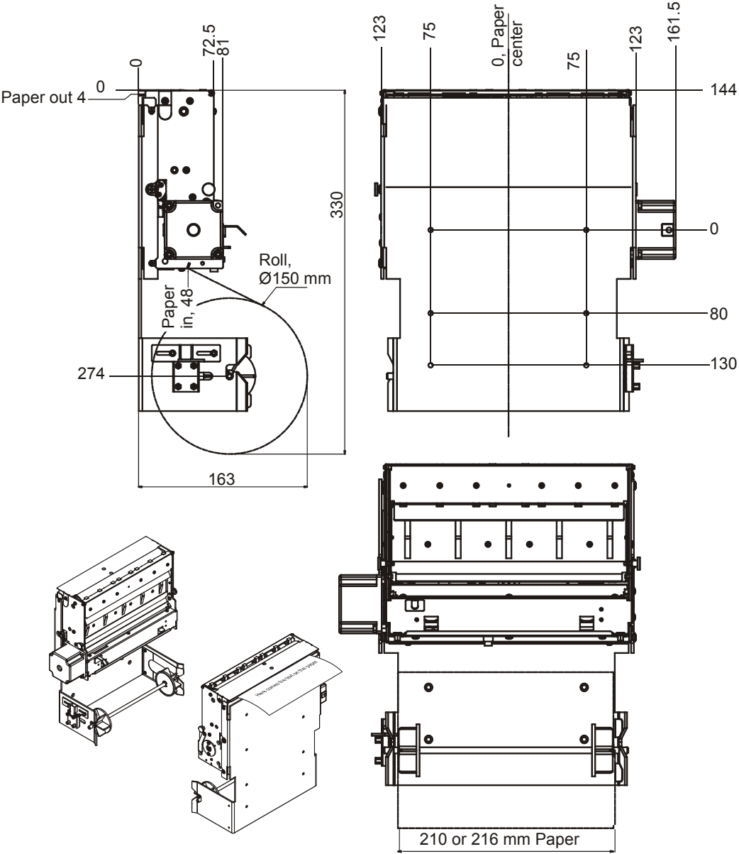
Figure 24 • Measurements Drawing, Vertical Printer 01760-xxx with Combo Roll Holder 01861-21x for 150 mm Roll Under Printer
