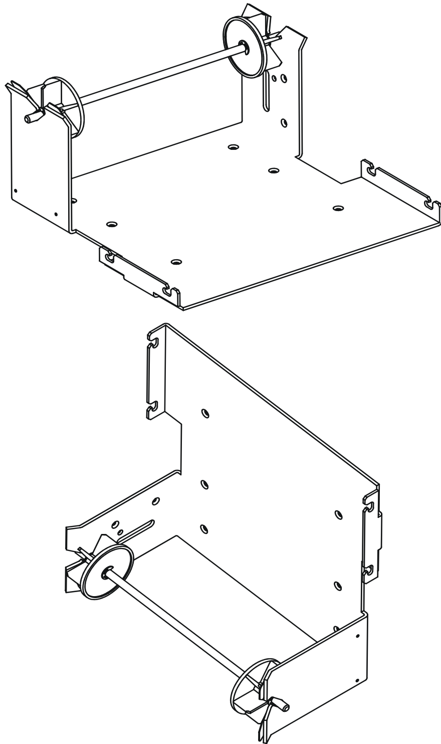
Figure 26 • Combo Roll Holder 01861-21x for Standard, Compact, and Vertical Versions of the Printer
