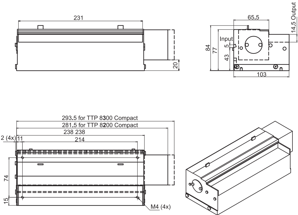
Figure 23 • Measurements Drawing, Compact Printer 01755-XXX
