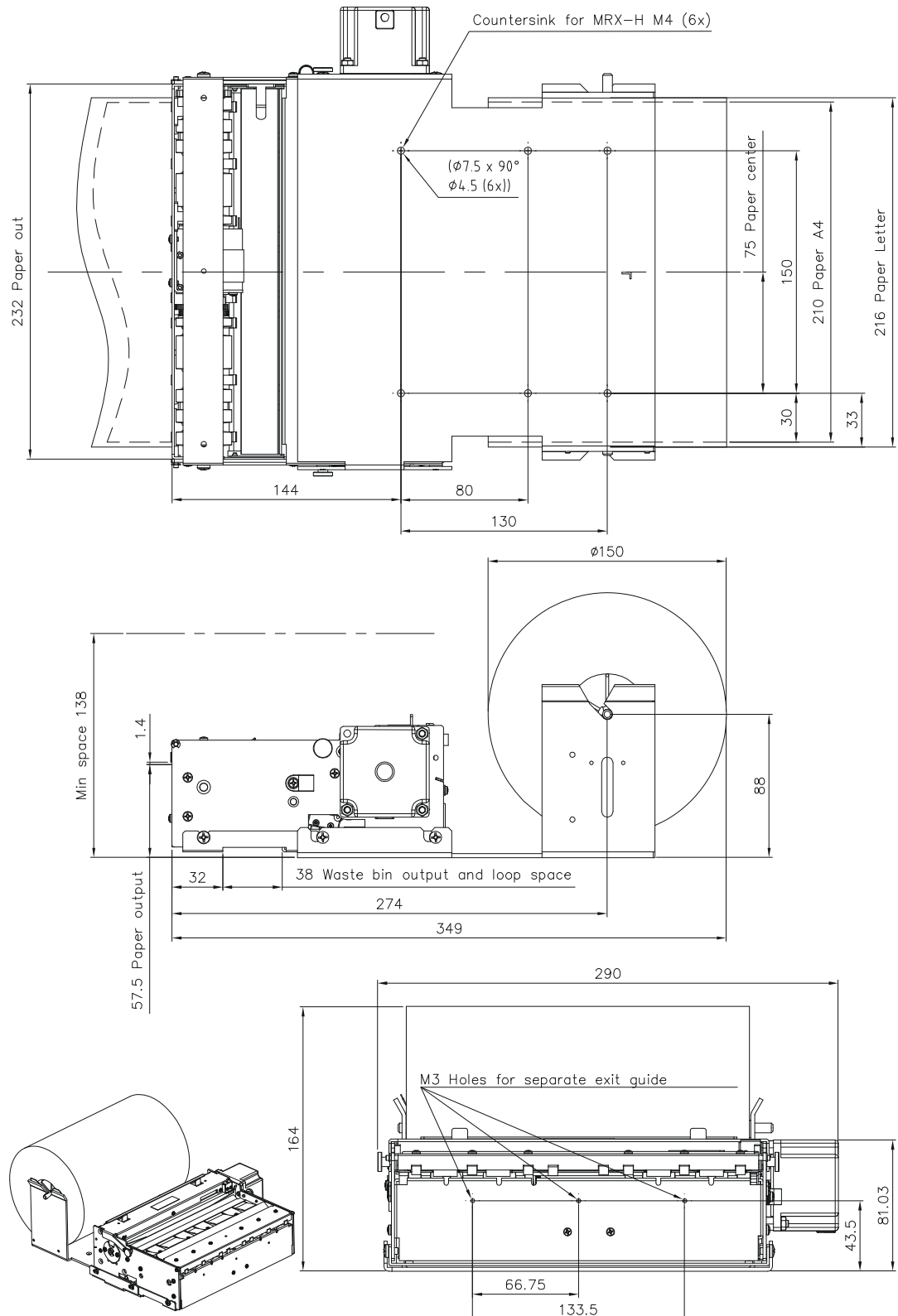
Figure 27 • Measurements Drawing, Printer 01744-xxx with Combo Roll Holder 01861-21x for up to 150mm Roll Behind
