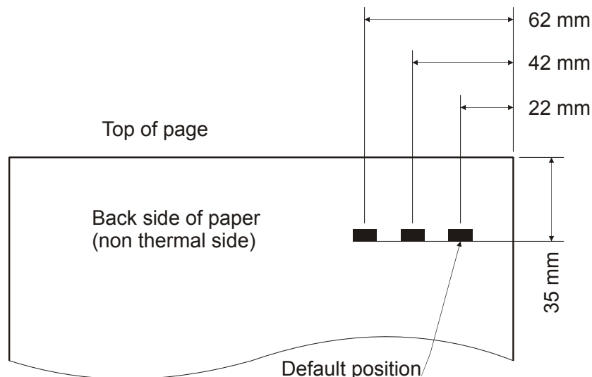
Figure 30 • Recommended Black Mark Print on Back of Paper (Only the “22 mm Mark”)
