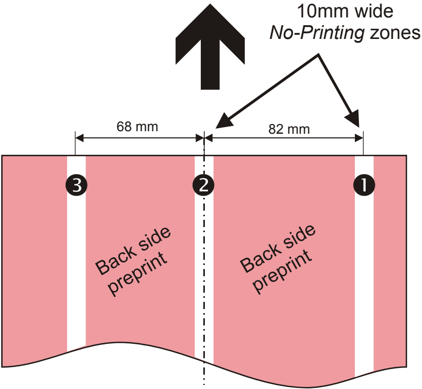
Figure 29 • Forbidden Print Zones
