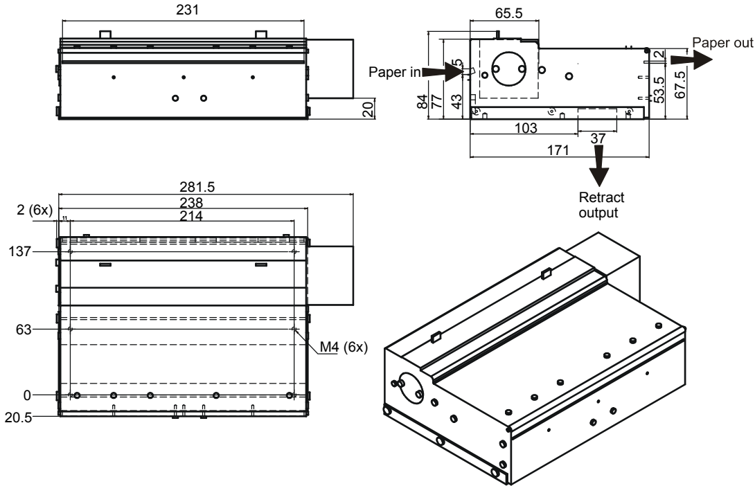
Figure 22 • Measurements Drawing, Standard Printer 01744-xxx and 01745-xxx
