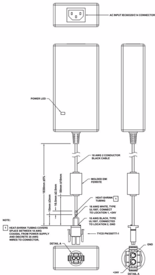
Figure 25 • 100W Power Supply
