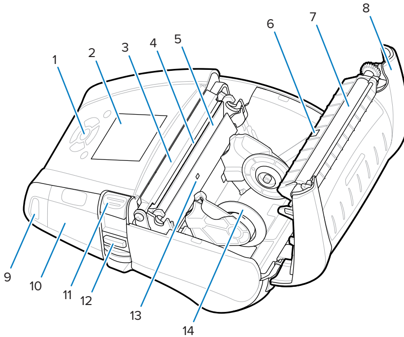
Figure 4 Printer Components - Overhead View (ZQ630 Plus)
