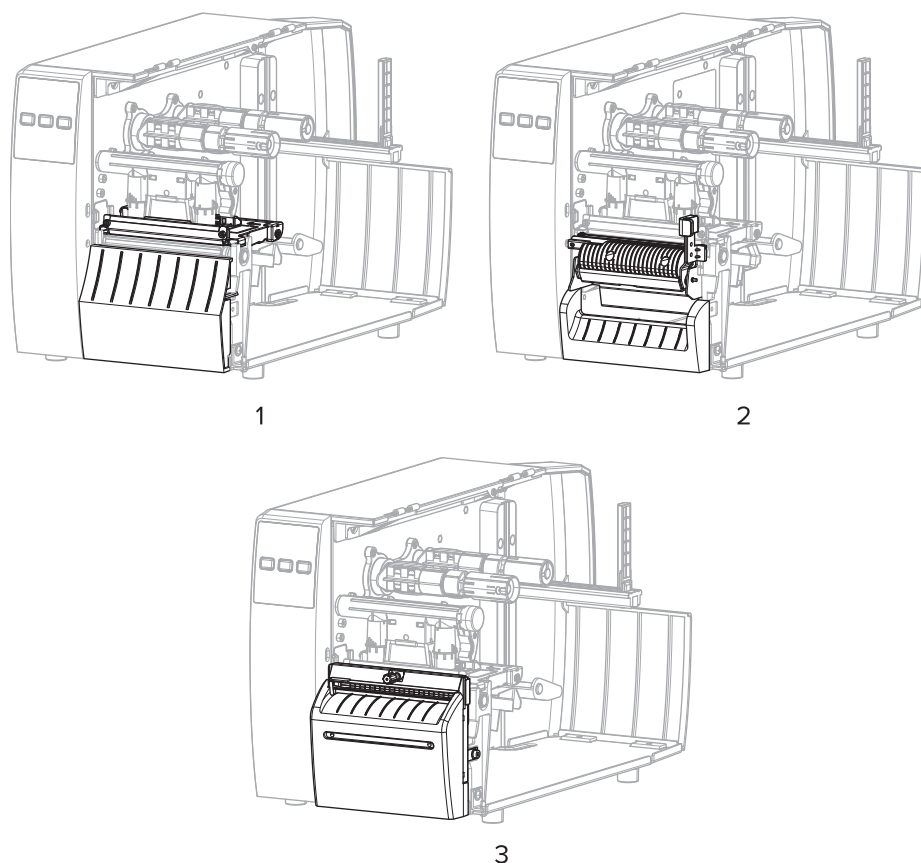
Figure 3 Printer Options
