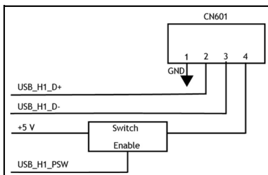
Figure 7-2 Workabout Pro G2 and Workabout Pro3 Internal USB Connector Block Diagram
