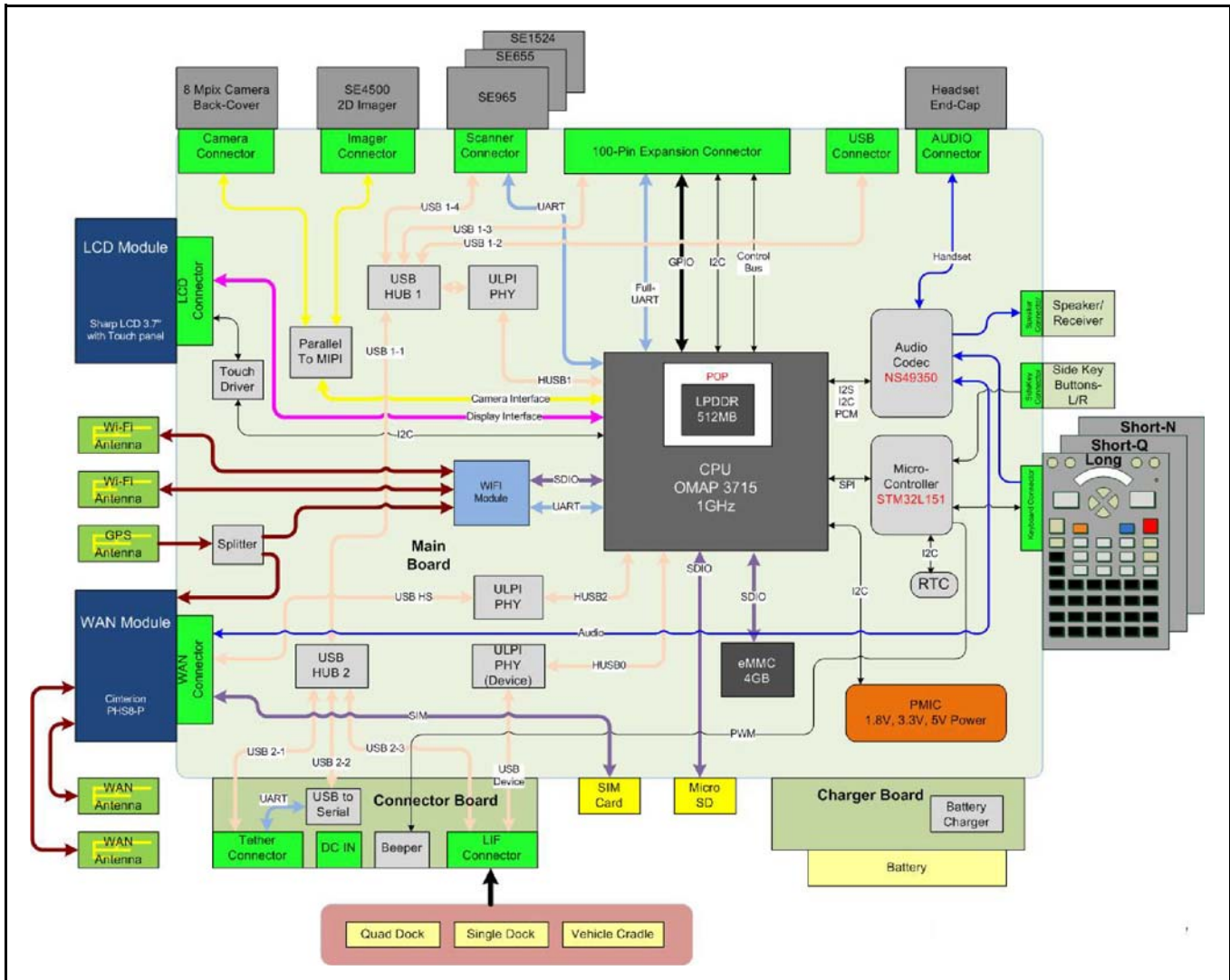
Figure 1-3 Workabout Pro4 Block Diagram
