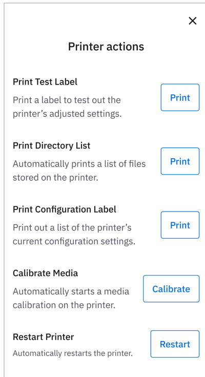
Figure 6 Printer Actions
