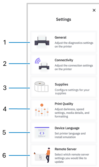
Figure 2 Settings Menu
