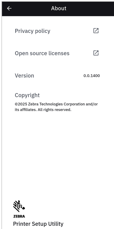
Figure 16 About Zebra
