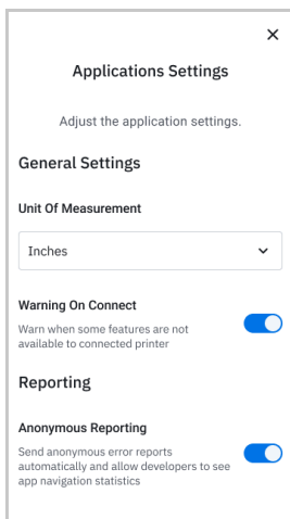
Figure 12 Application Settings
