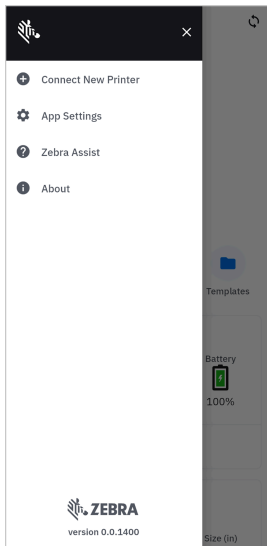
Figure 11 Side-Drawer Menu
