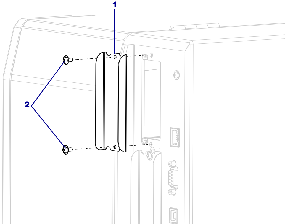
Figure 11 • Remove the Blank Cover (ZT600 Shown)
