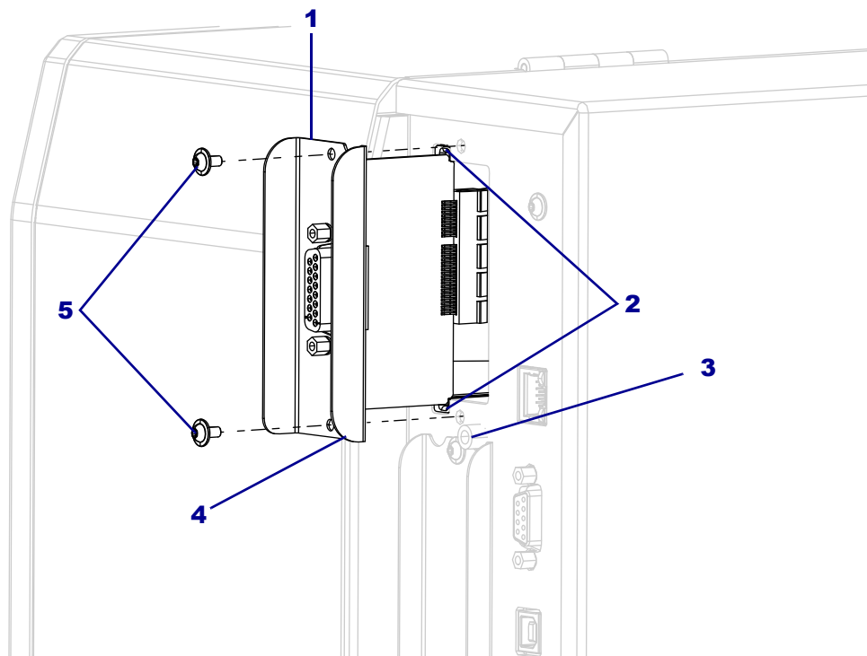
Figure 12 • Install the Applicator Interface Card (ZT600 shown)
