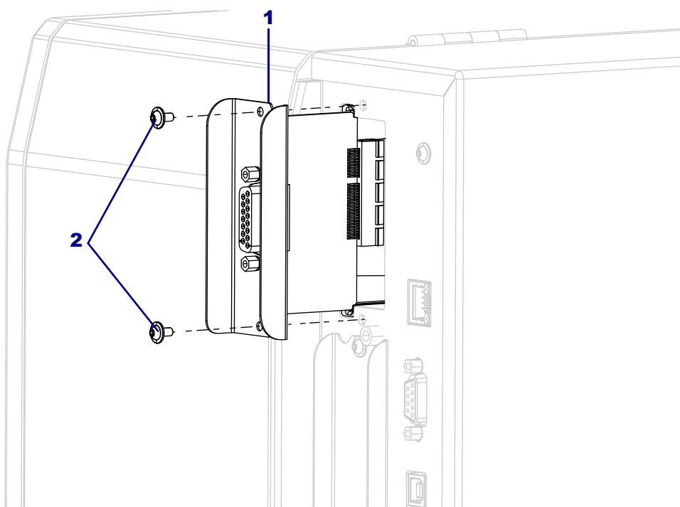
Figure 10 • Remove the Option Card (ZT600 Shown)
