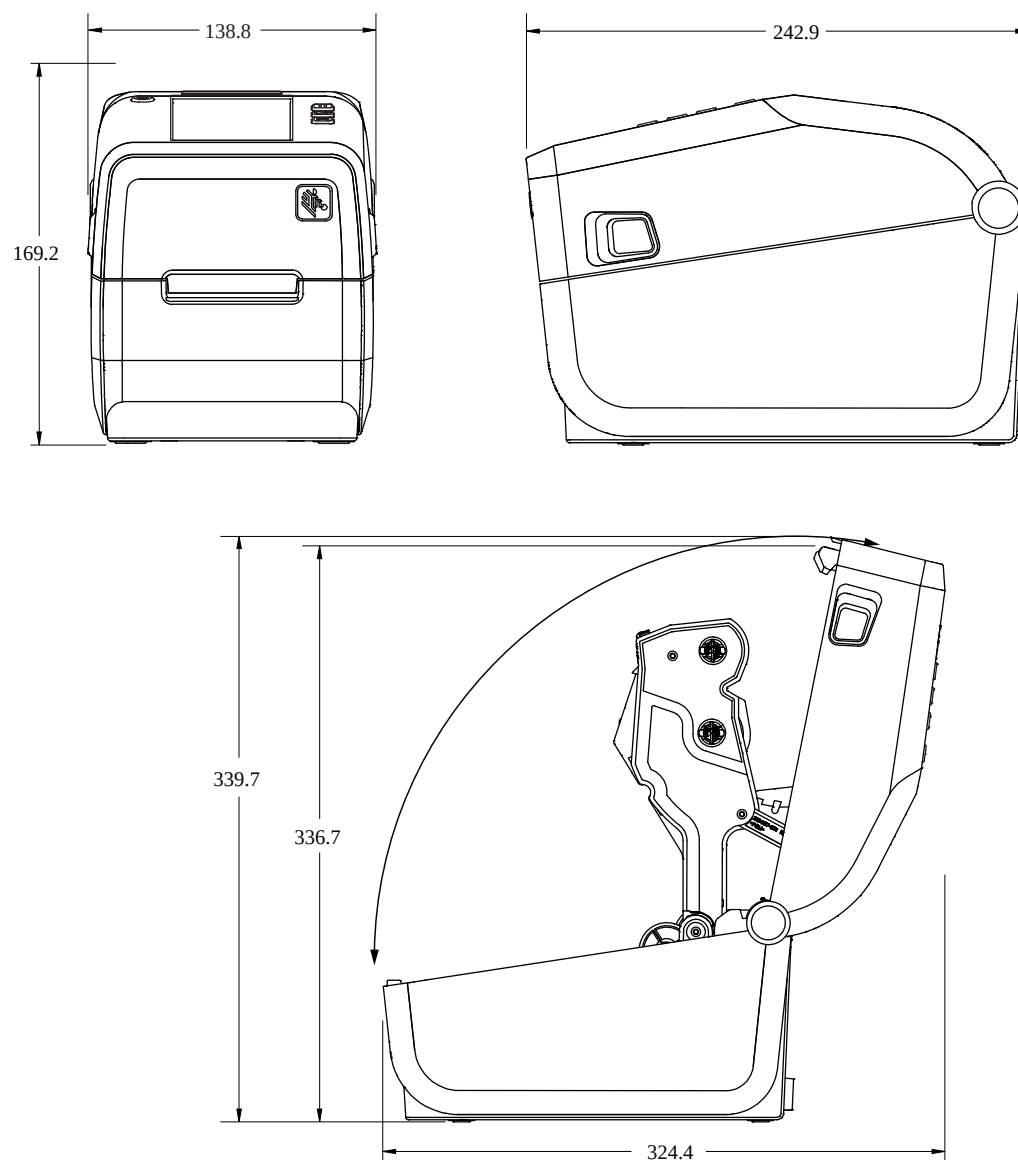
Figure 23 Imprimante standard ZD611R
