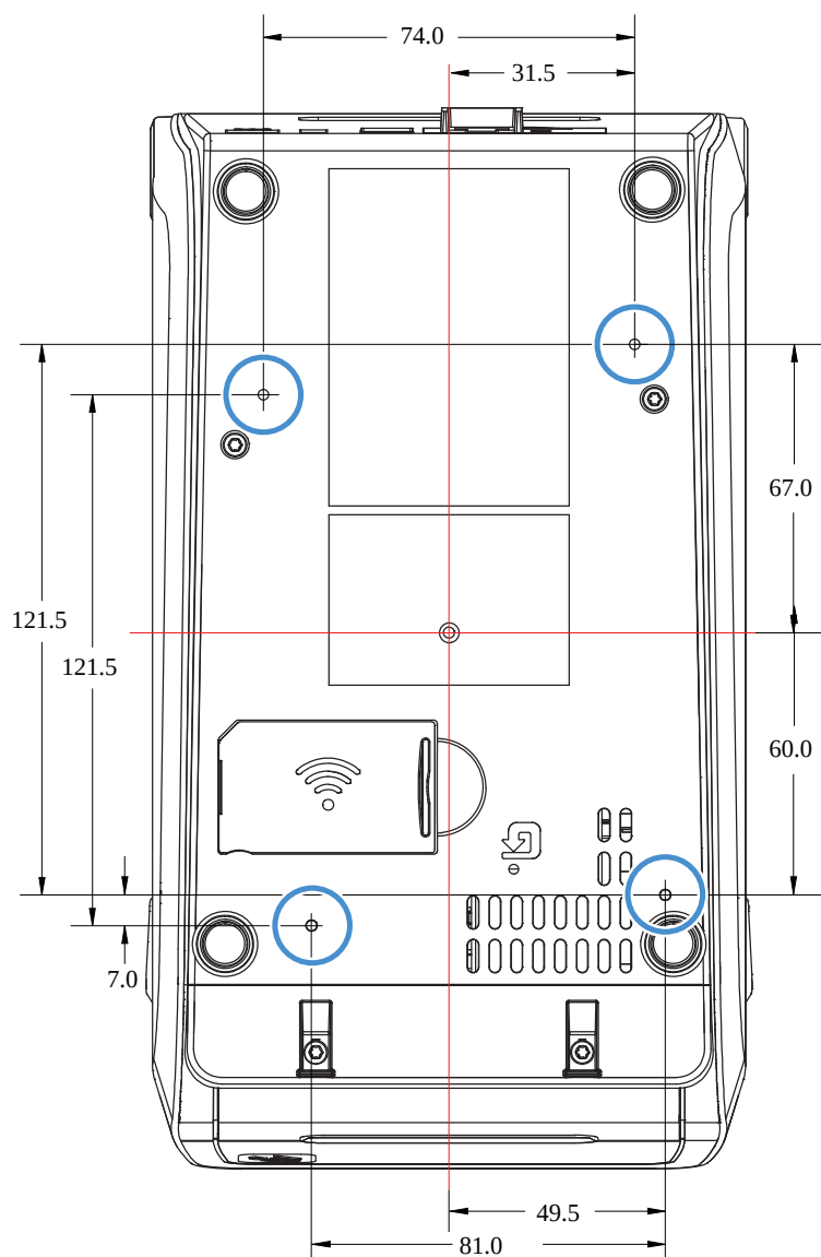
Figure 27 Montage standard ZD611R
