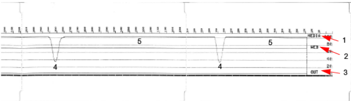
Figura 12 Sensor Profile (Black Mark, Tag Media)
