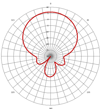
Vertical (FCC)
