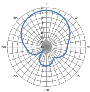
Horizontal (FCC)
