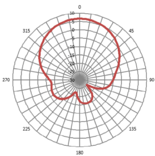
Vertical (FCC)
