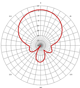
Vertical (FCC)
