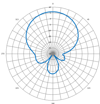
Horizontal (FCC)
