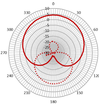
Horizontal (FCC)
