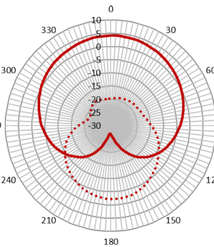
Vertical (FCC)
