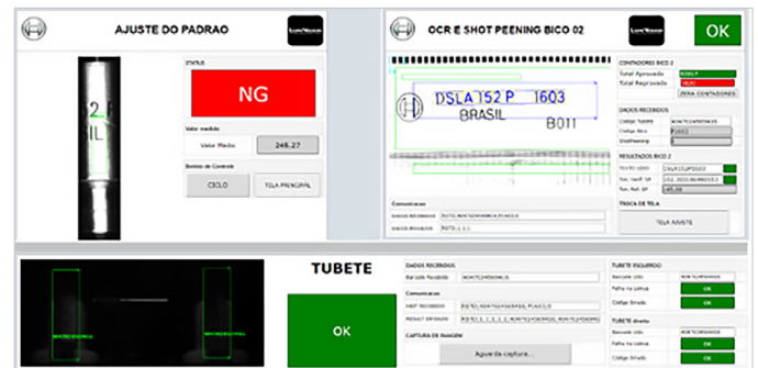
Screen showing the necessary adjustments to build unwrapped image with segments of injector cylinder.
