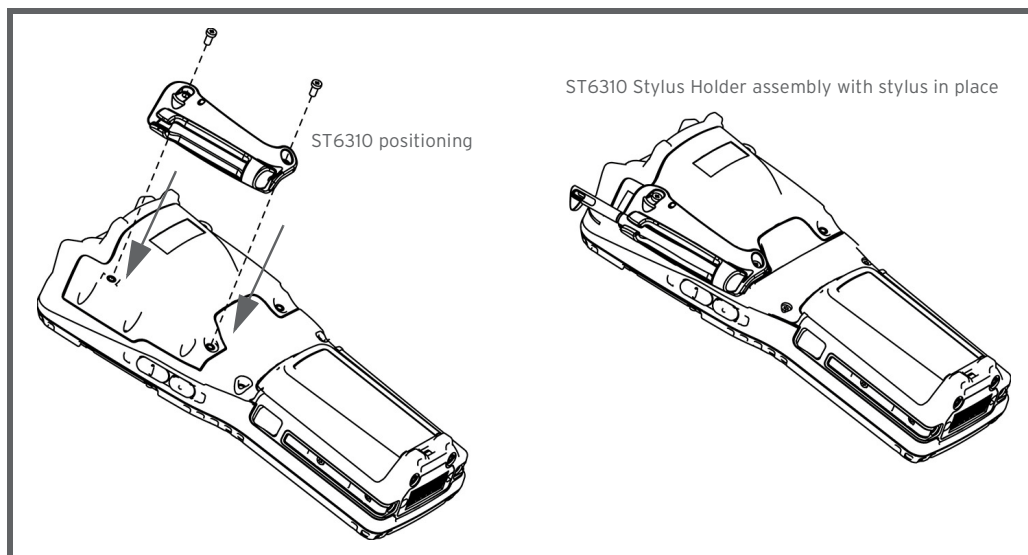
Figure 1 Attaching the Stylus Holder
