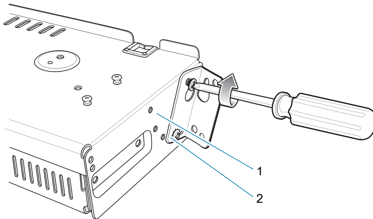
Figure 77 Flange 25° Position (4-Slot Battery Chargers)
