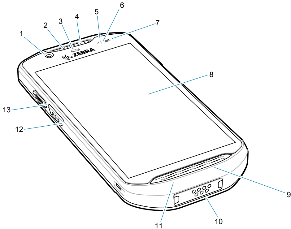
Figure 5 TC52ax-HC Front View
