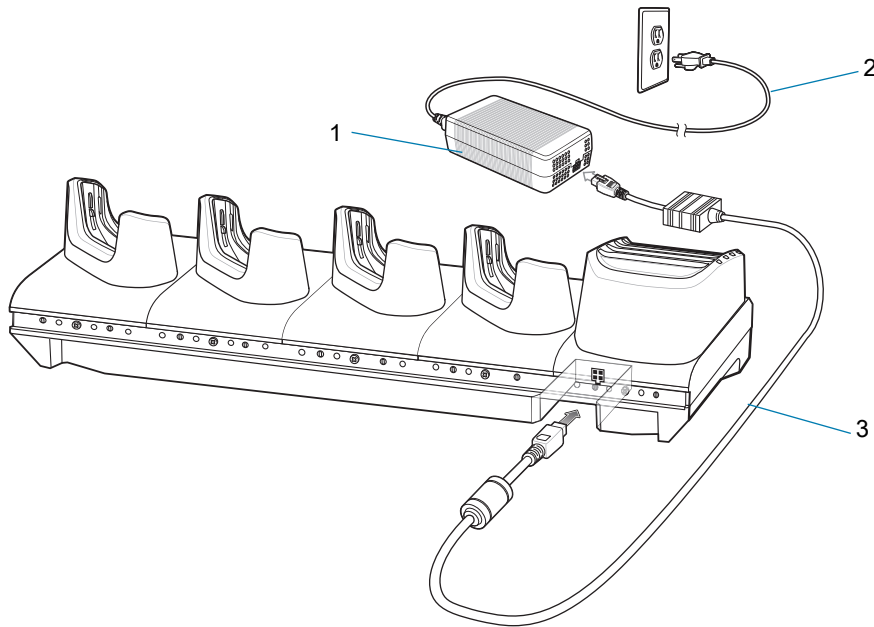
Figure 64 4-Slot Charge Only Cradle with Battery Charger Setup
