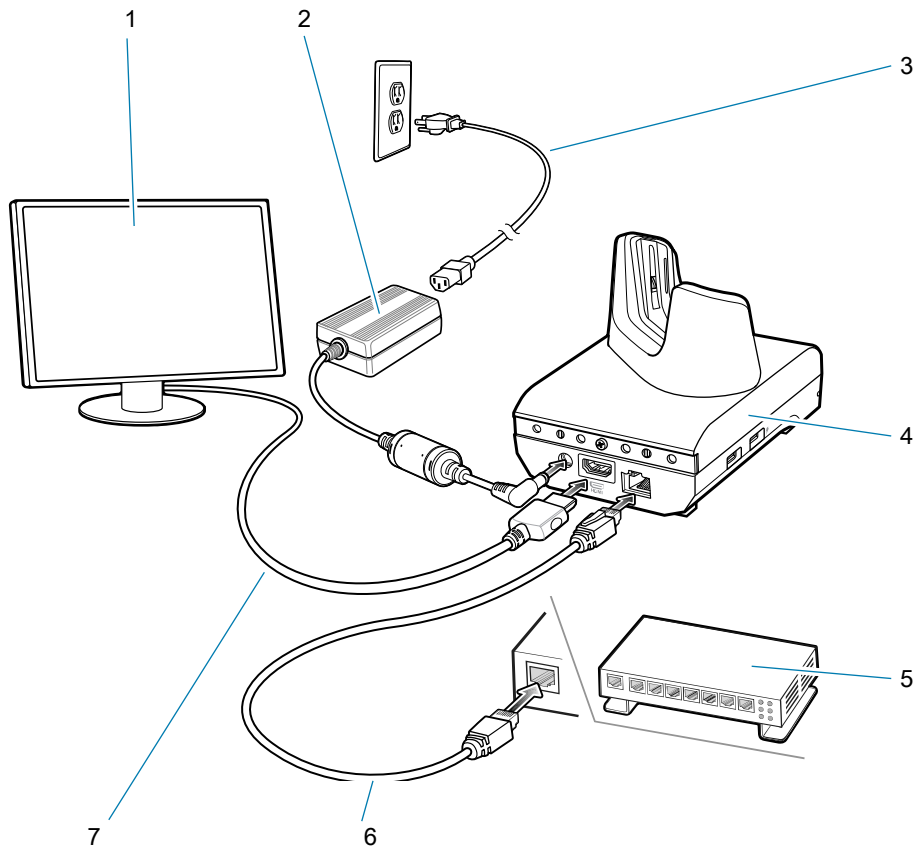
Figure 56 Workstation Cradle Setup
