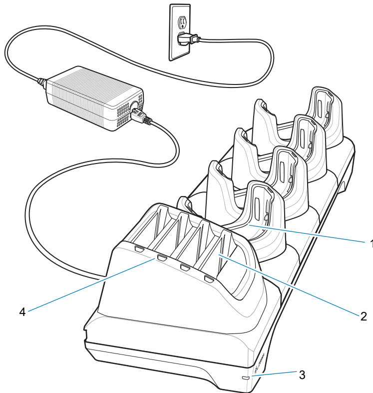
Figure 63 4-Slot Charge Only Cradle with Battery Charger
