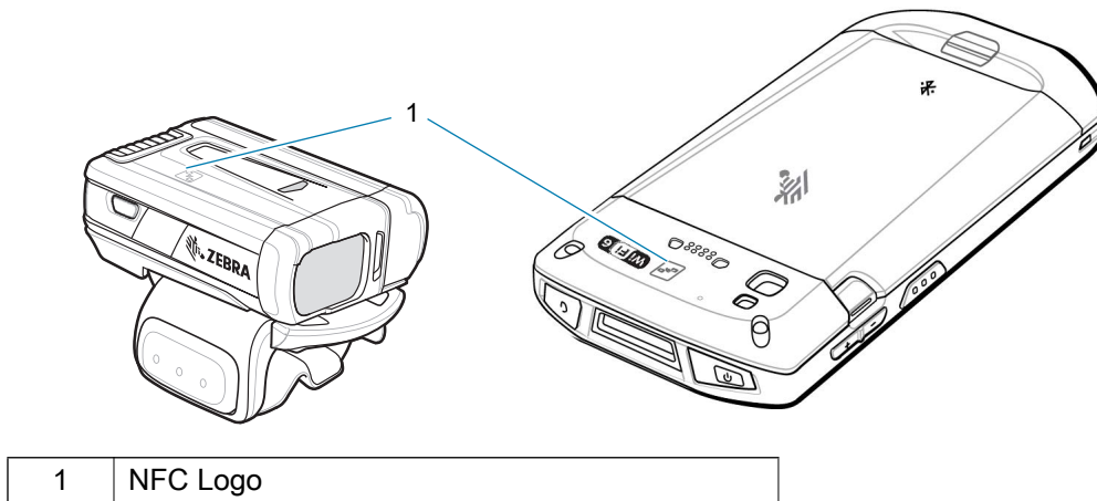
Figure 44 Align NFC Antennas (RS6000 shown)
