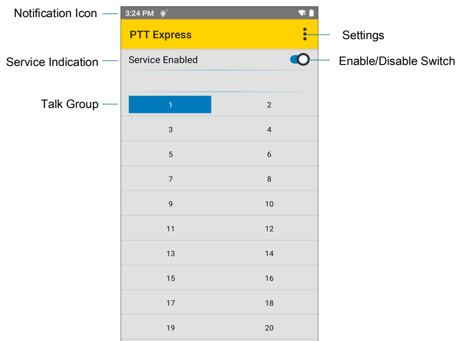
Figure 15 PTT Express Default User Interface
