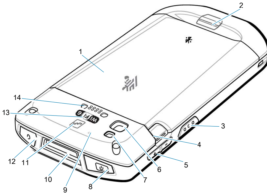
Figure 4 TC52ax Advanced Range Rear View
