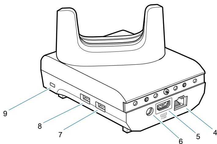
Figure 55 Rear/Right Side View
