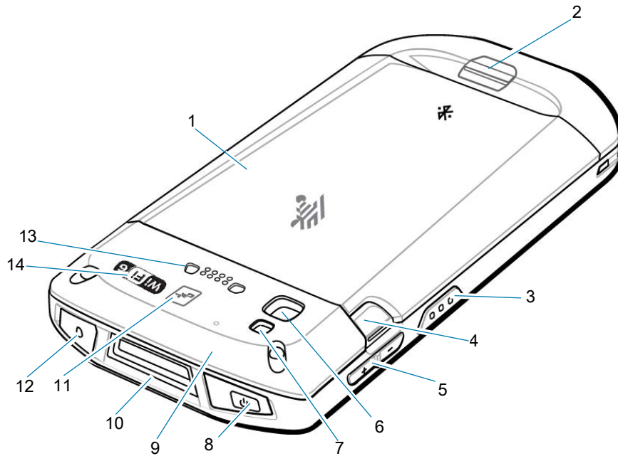
Figure 2 TC52ax Standard Rear View
