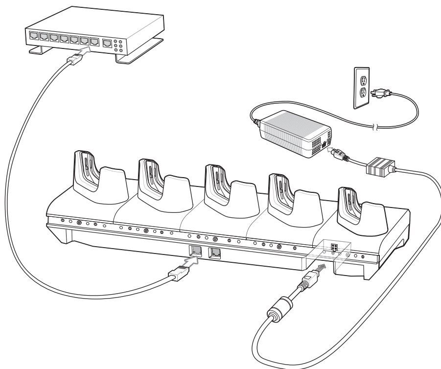
Figure 70 5-Slot Ethernet Cradle Setup
