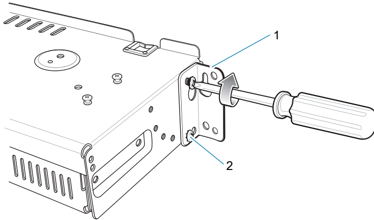
Figure 76 Flange Horizontal Position (5-Slot Cradles)
