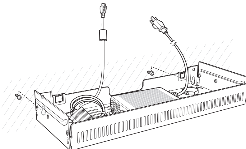
Figure 79 Horizontal Installation
