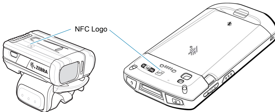
Figure 45 Align NFC Antennas (RS6000 shown)
