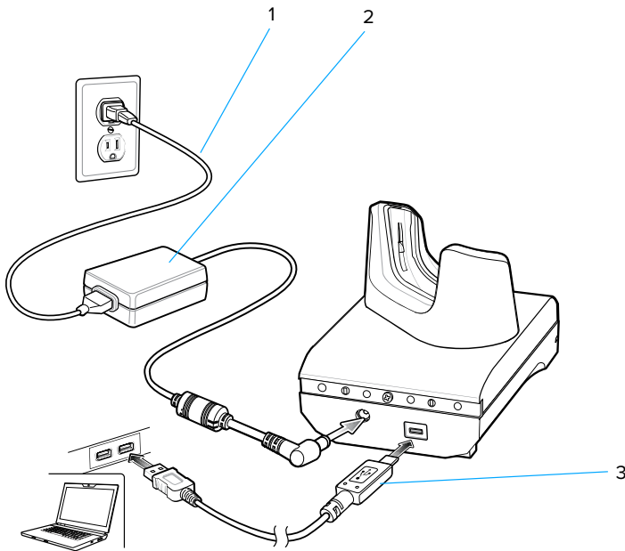
Figure 51 1-Slot USB Charge Cradle Setup
