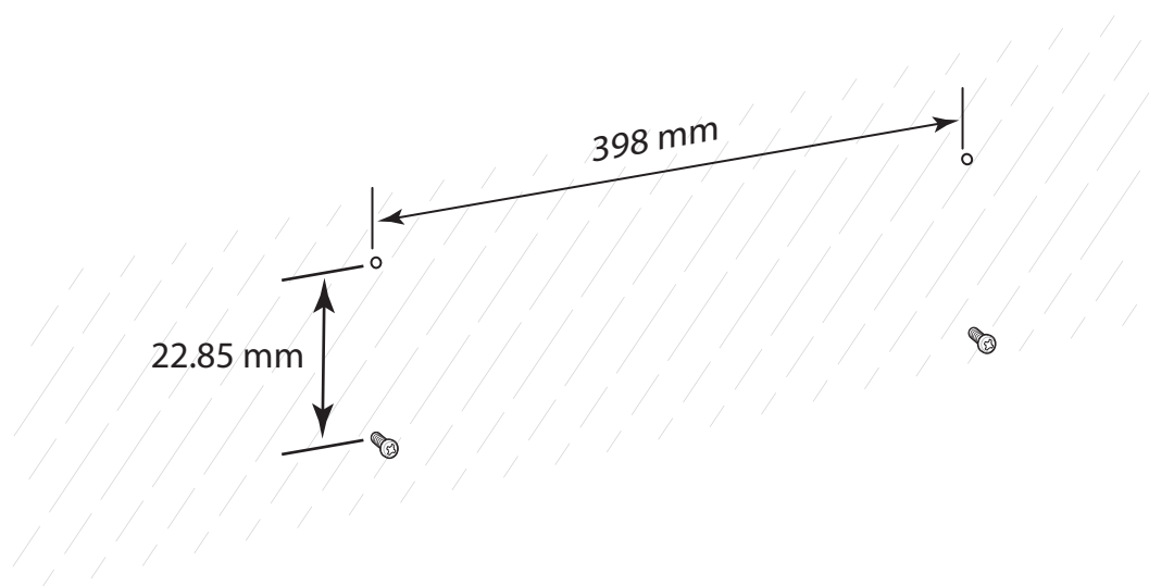
Figure 78 Horizontal Mounting Template
