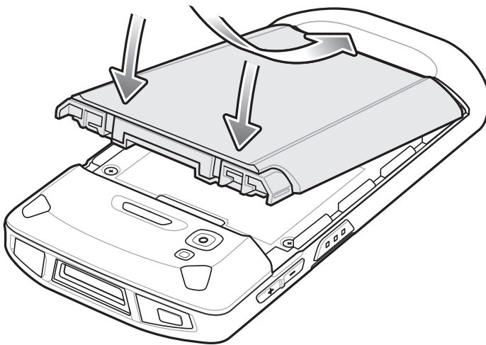
Figure 16 Insert Bottom of Battery into Battery Compartment
