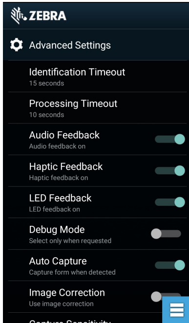
Figure 101 Advanced Settings Screen
