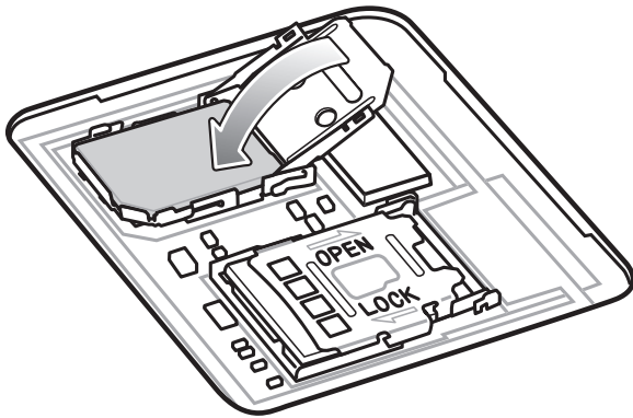
Figure 13 Close SIM Card Holder Door
