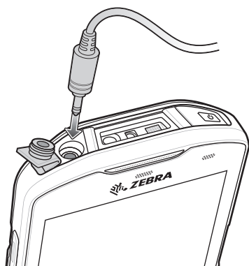
Figure 159 Audio Adapter Installation
