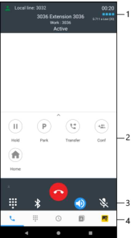
Figure 15 In-Call Dashboard
