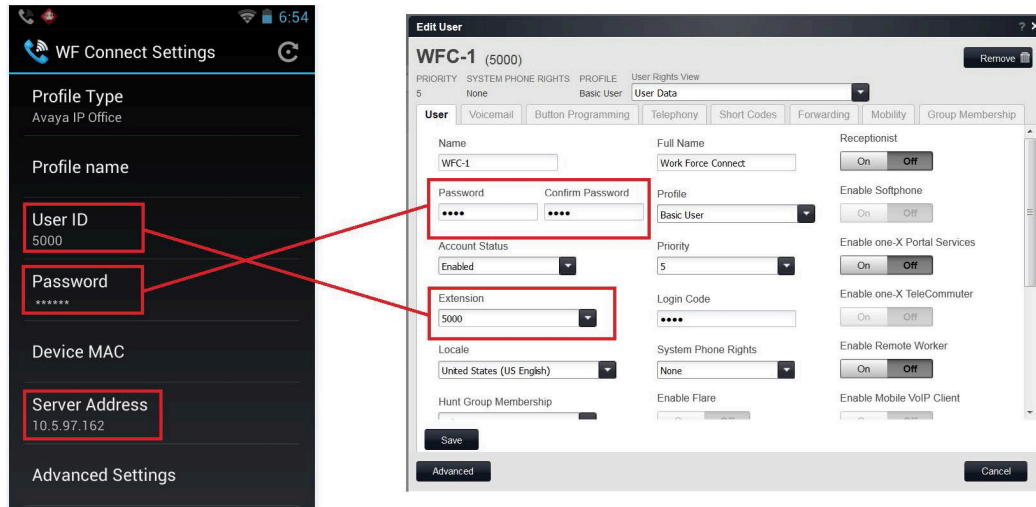
Figure 1 Device Settings
