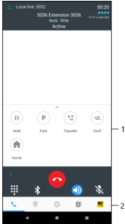
Figure 9 In-Call Dashboard
