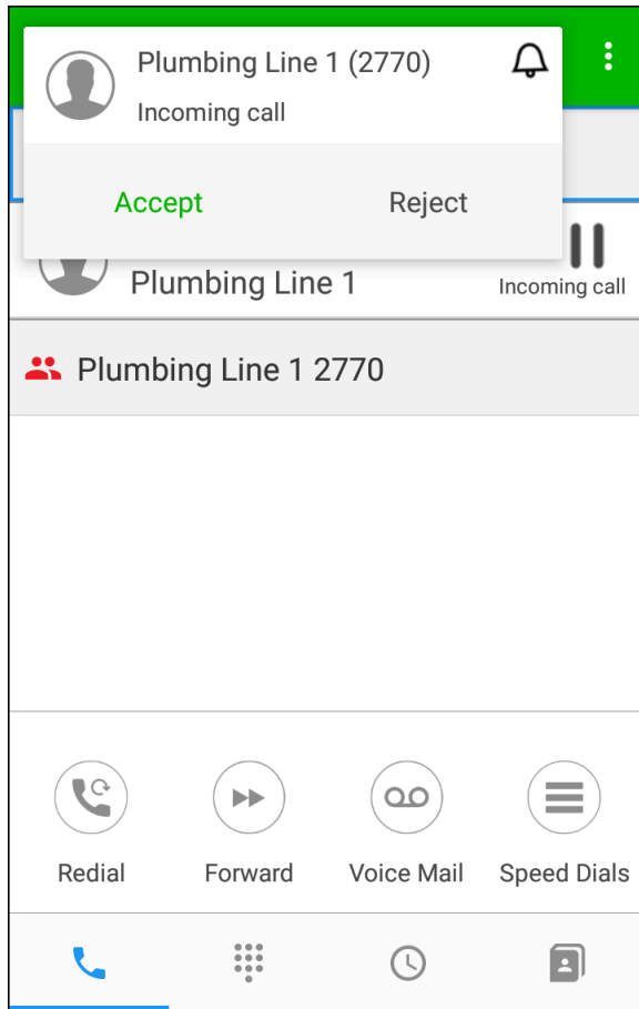
Figure 15 Popup Window
