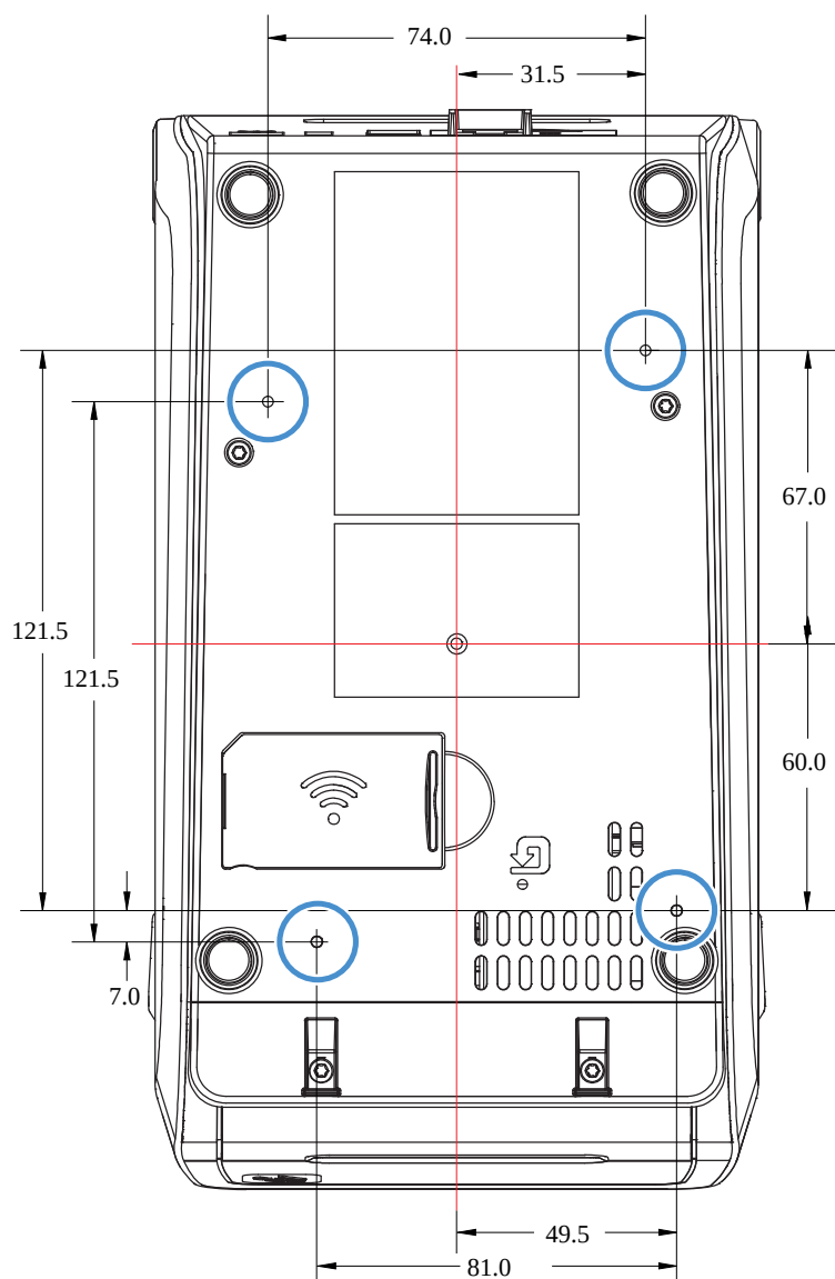
Figure 20 Montage standard ZD611T
