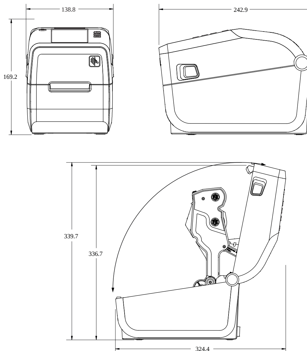
Figure 16 Imprimante standard ZD611T
