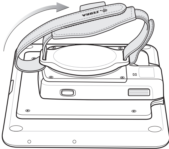
Figure 2-46 Secure Strap
