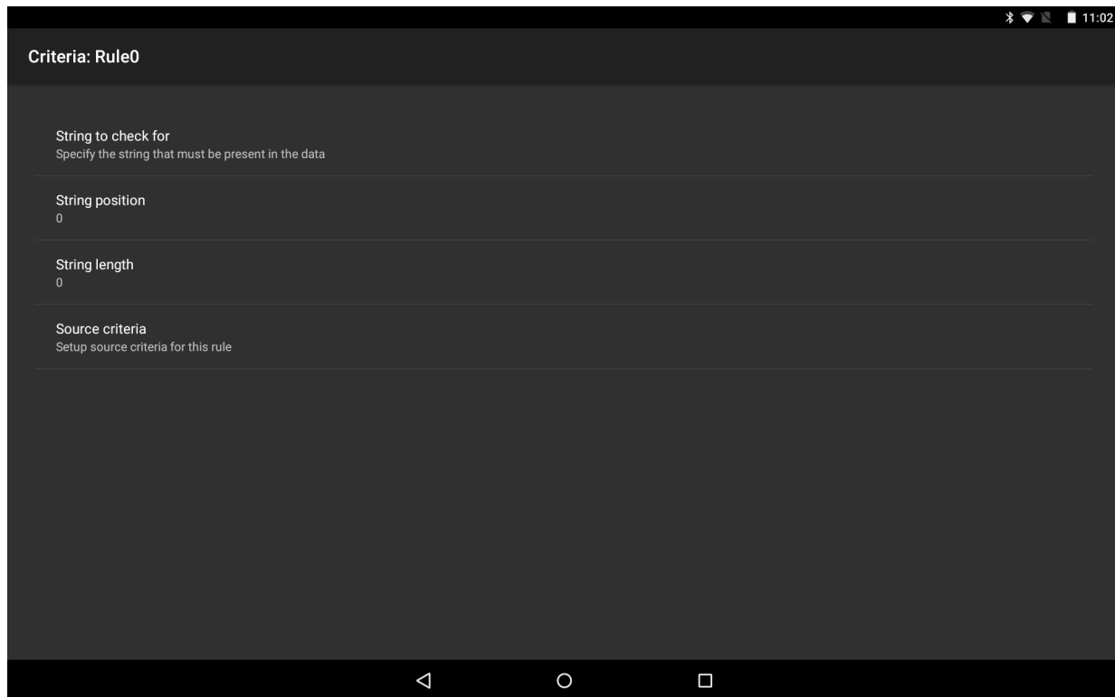
Figure 4-22 Criteria Screen
