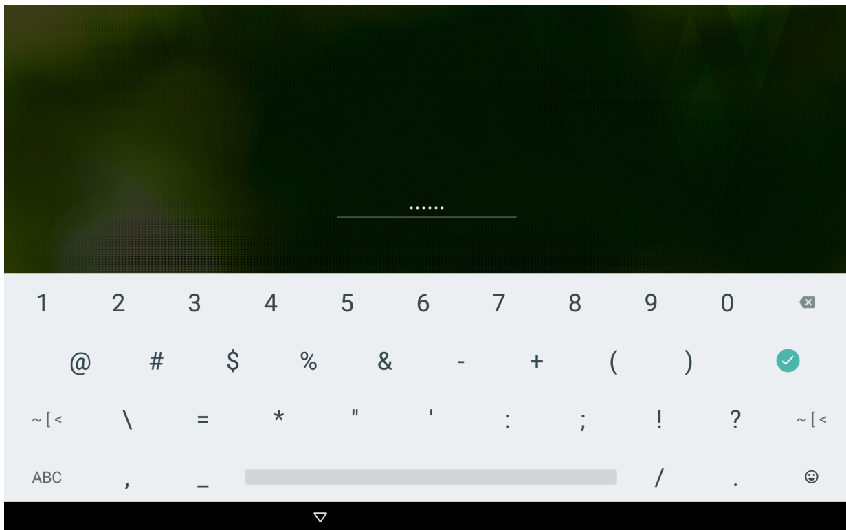
Figure 5-2 Password Screen
