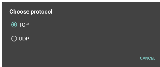
Figure 4-18 Protocol Selection
