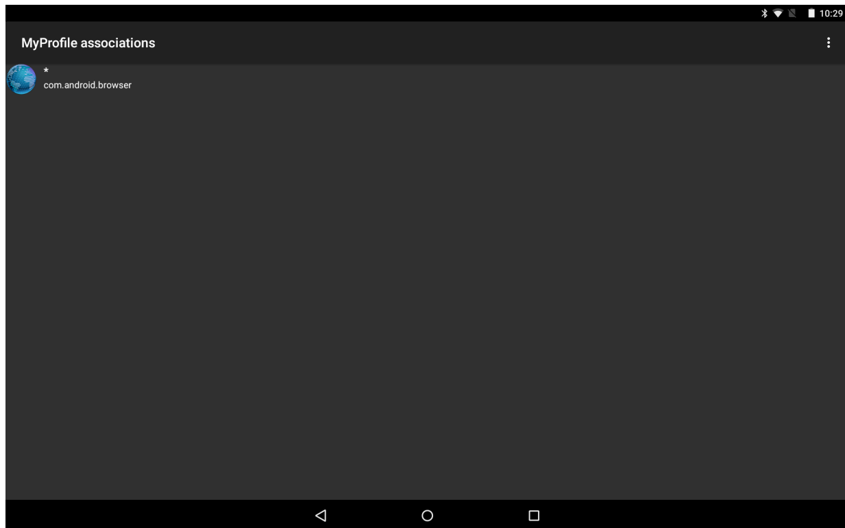
Figure 4-10 Selected Application/Activity
