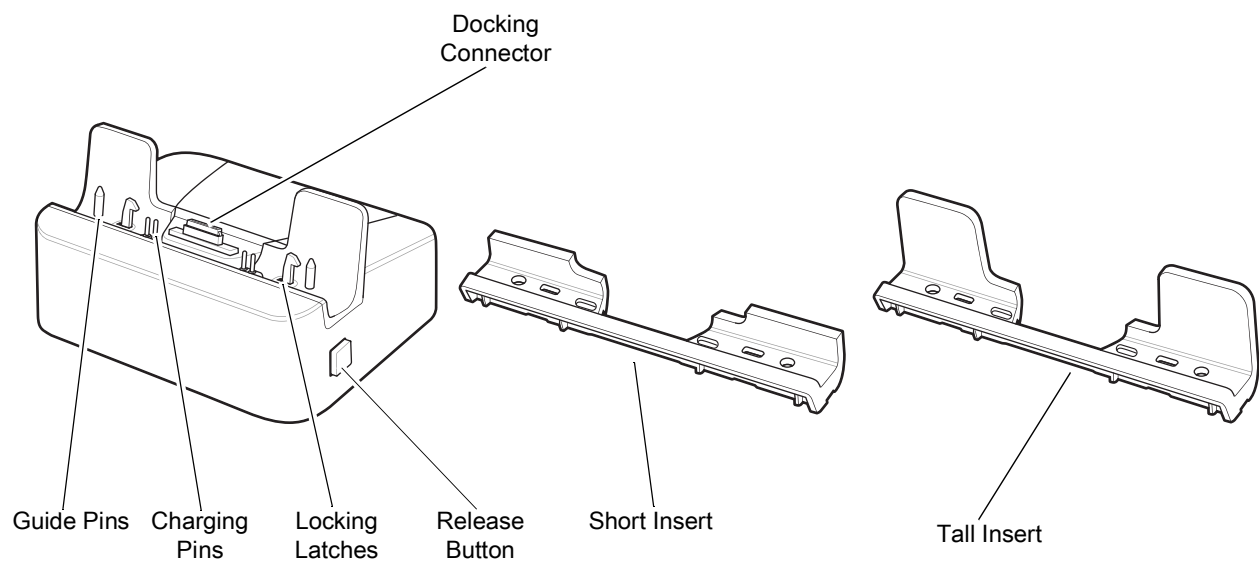
Figure 2-6 Communication and Charging Cradle - Front View
