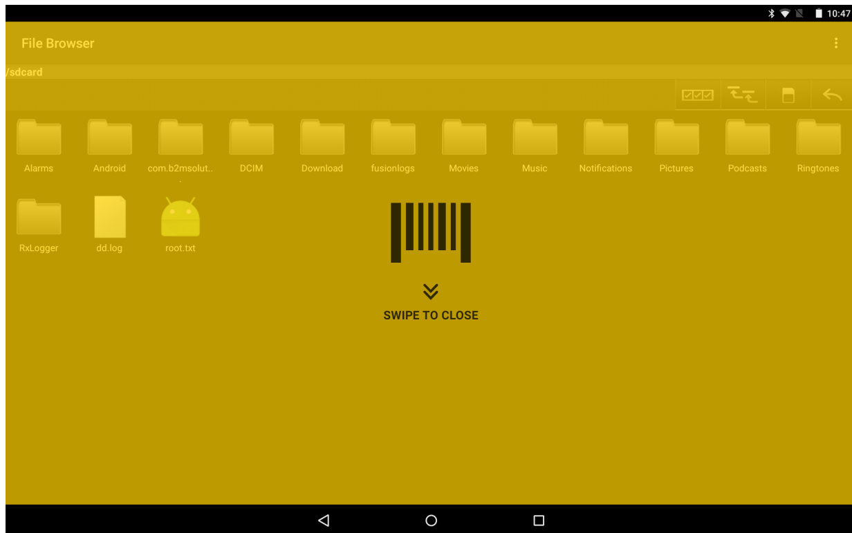
Figure 4-13 Fullscreen Mode
