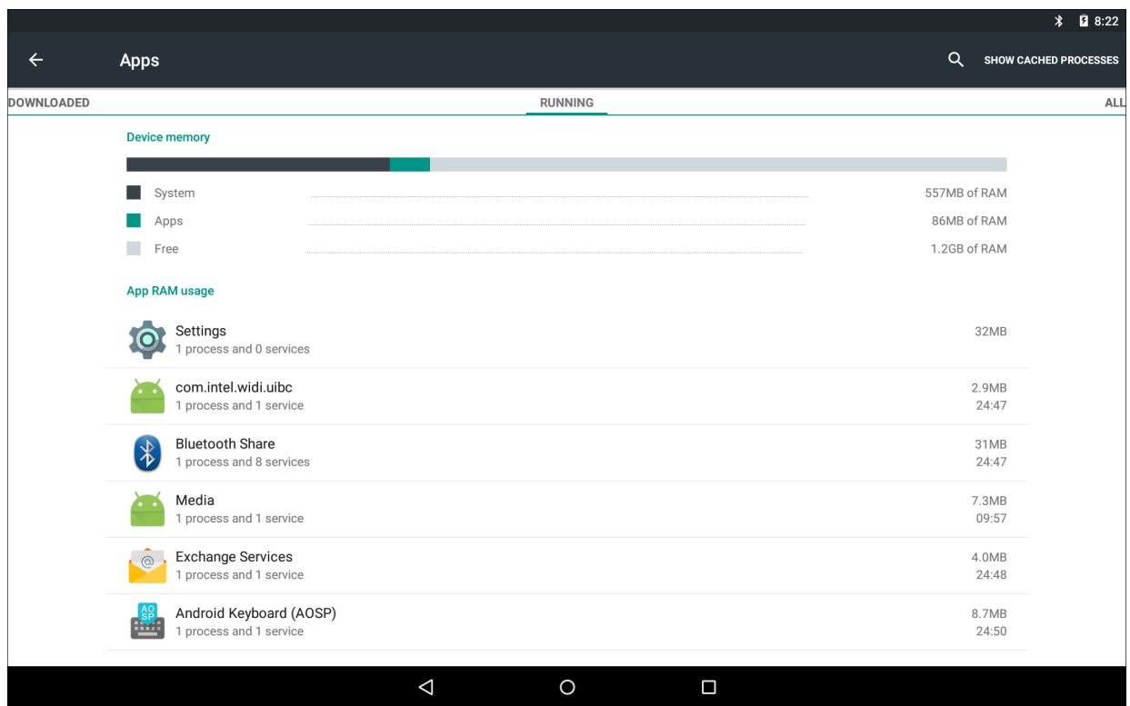
Figure 6-2 Running Screen
