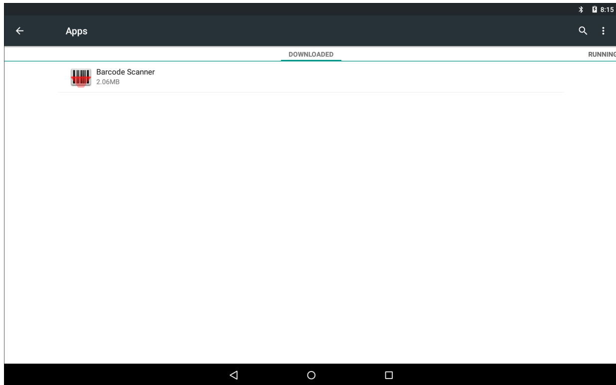
Figure 6-1 Downloaded Screen
