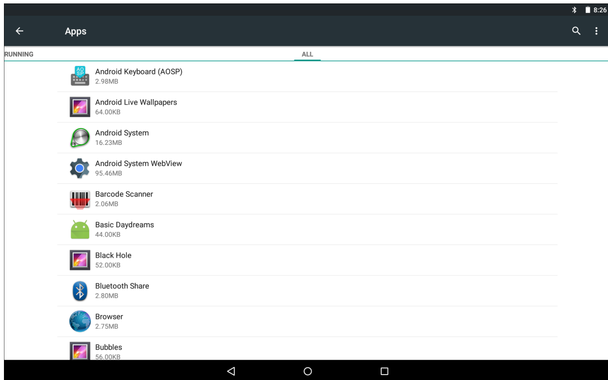
Figure 6-6 Apps Screen
