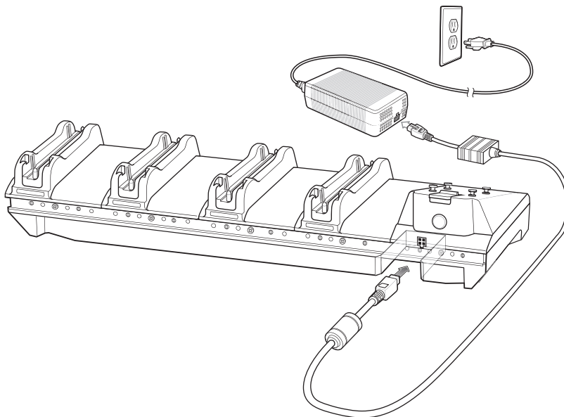
Figure 2-22 4-Slot Charge Only Cradle Setup
