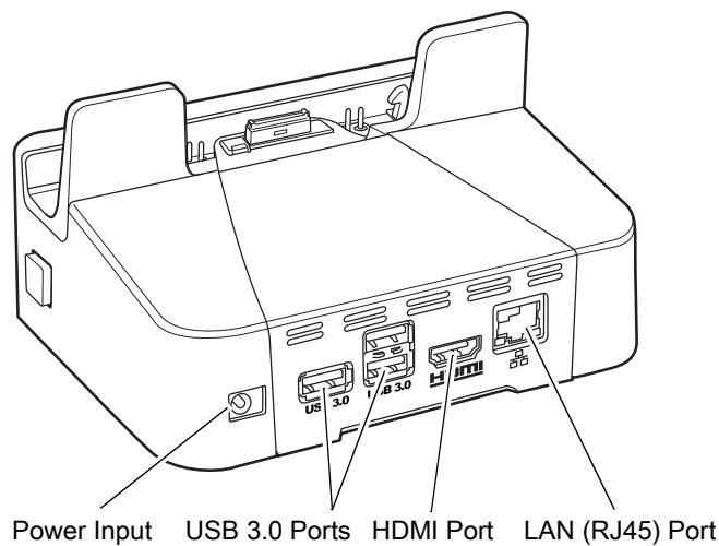
Figure 2-7 Communication and Charging Cradle - Rear View
