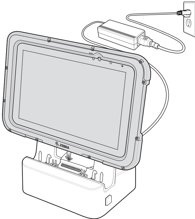
Figure 2-15 Insert ET5X with Rugged Frame and IO Adapter into Rugged Communication and Charging Cradle
