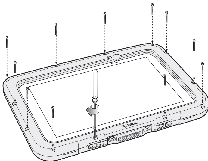
Figure 2-31 Secure 8" Rugged Frame
