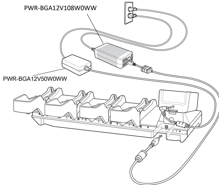
Figure 2-23 4-Slot Charge Only Cradle with Battery Charger Setup
