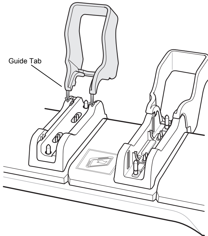
Figure 2-19 Align Guide with Slot
