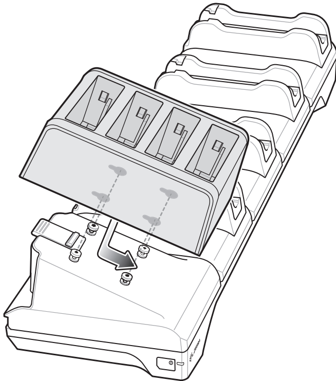
Figure 2-21 Align Battery Charger on Adapter
