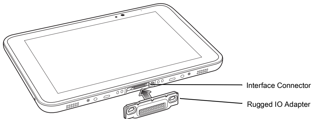
Figure 2-29 Insert Rugged IO Adapter
