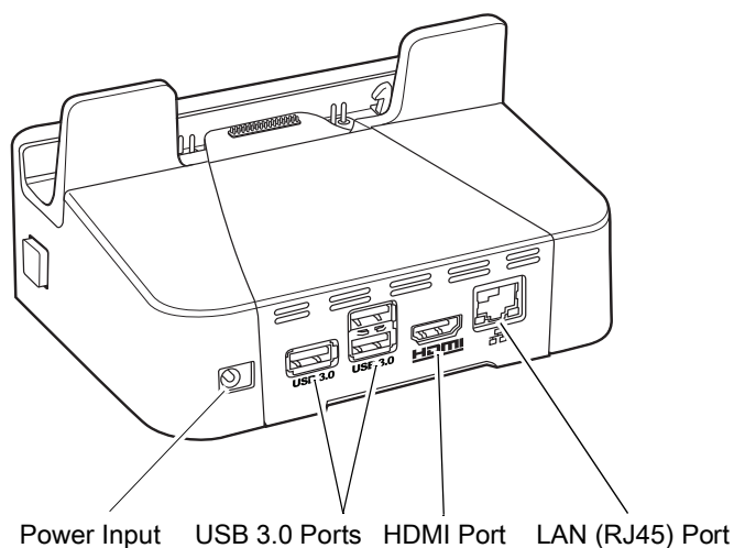
Figure 2-13 Rugged Communication and Charging Cradle - Rear View
