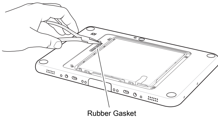
Figure 2-34 Remove Rubber Gasket
