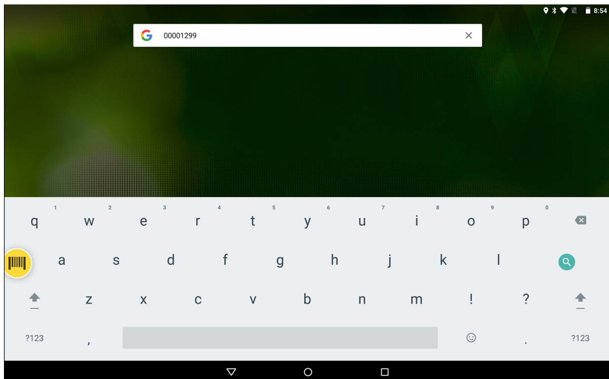
Figure 4-26 Formatted Data
