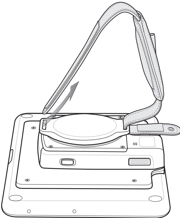
Figure 2-41 Remove Strap
