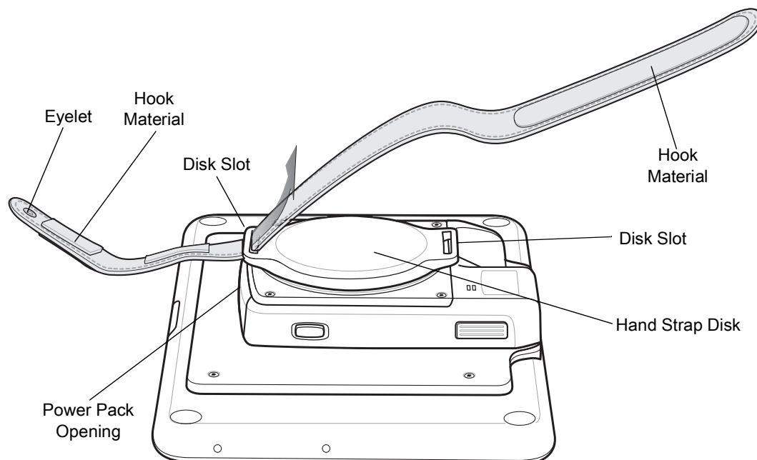
Figure 2-43 Feed New Strap
