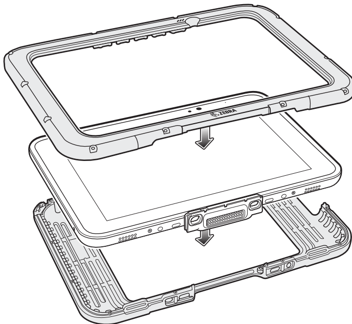
Figure 2-30 Protective Boot Assembly
