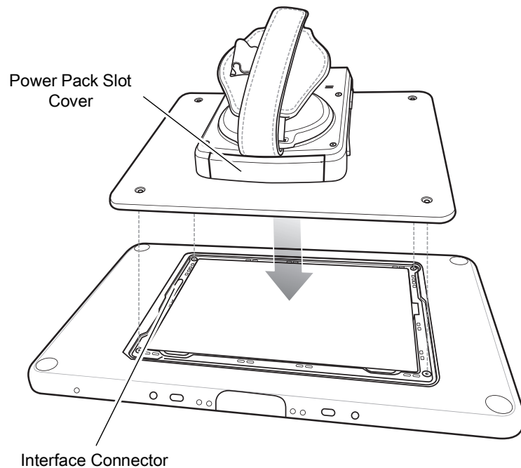
Figure 2-36 Align Expansion Back with 8" Configuration
