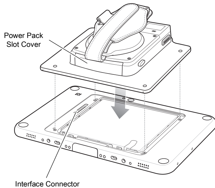
Figure 2-35 Align Expansion Back with 8" Configuration
