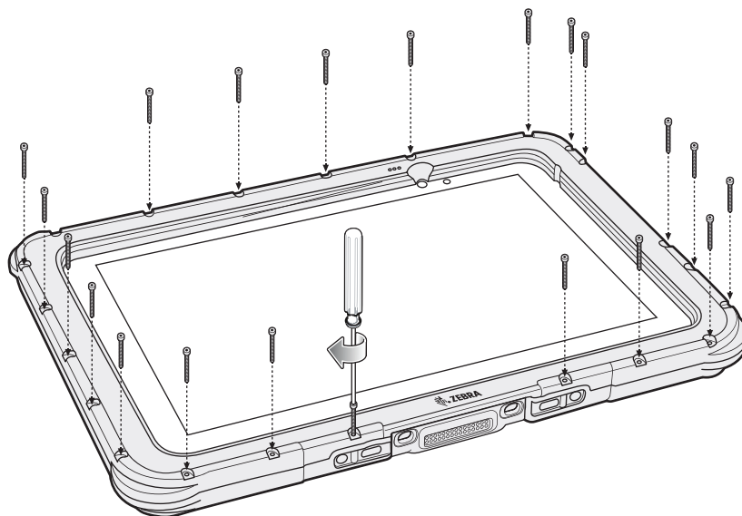
Figure 2-32 Secure 10" Rugged Frame
