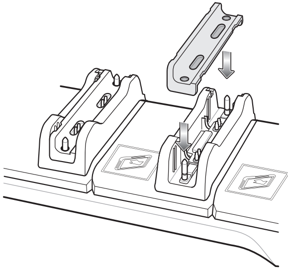
Figure 2-18 Install Insert in Slot
