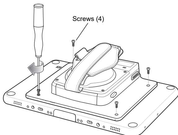
Figure 2-37 Secure Screws
