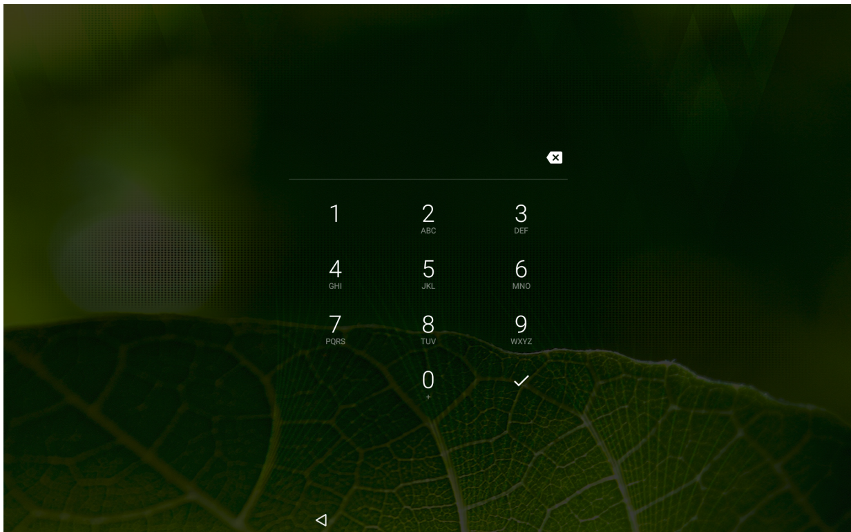
Figure 5-1 PIN Screen
