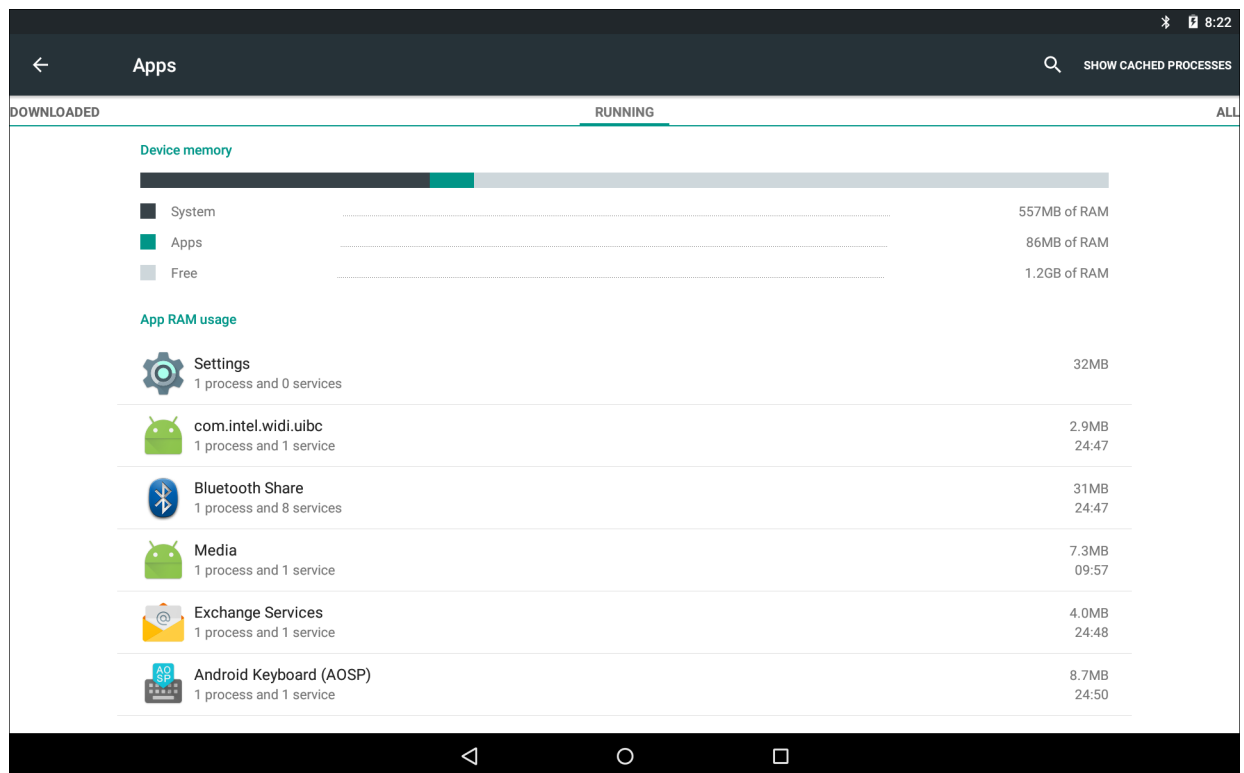
Figure 6-7 Running Applications
