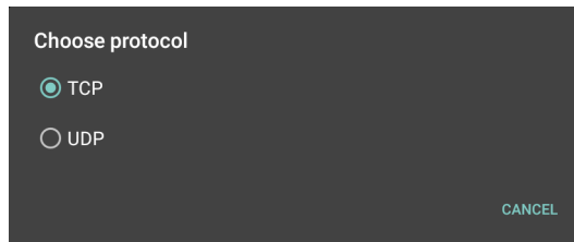
Figure 4-15 Protocol Selection
