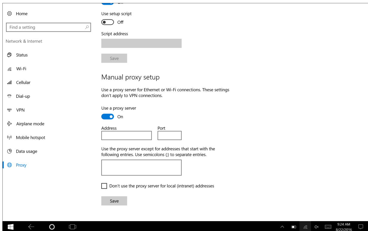
Figure 3-4 Proxy Setup
