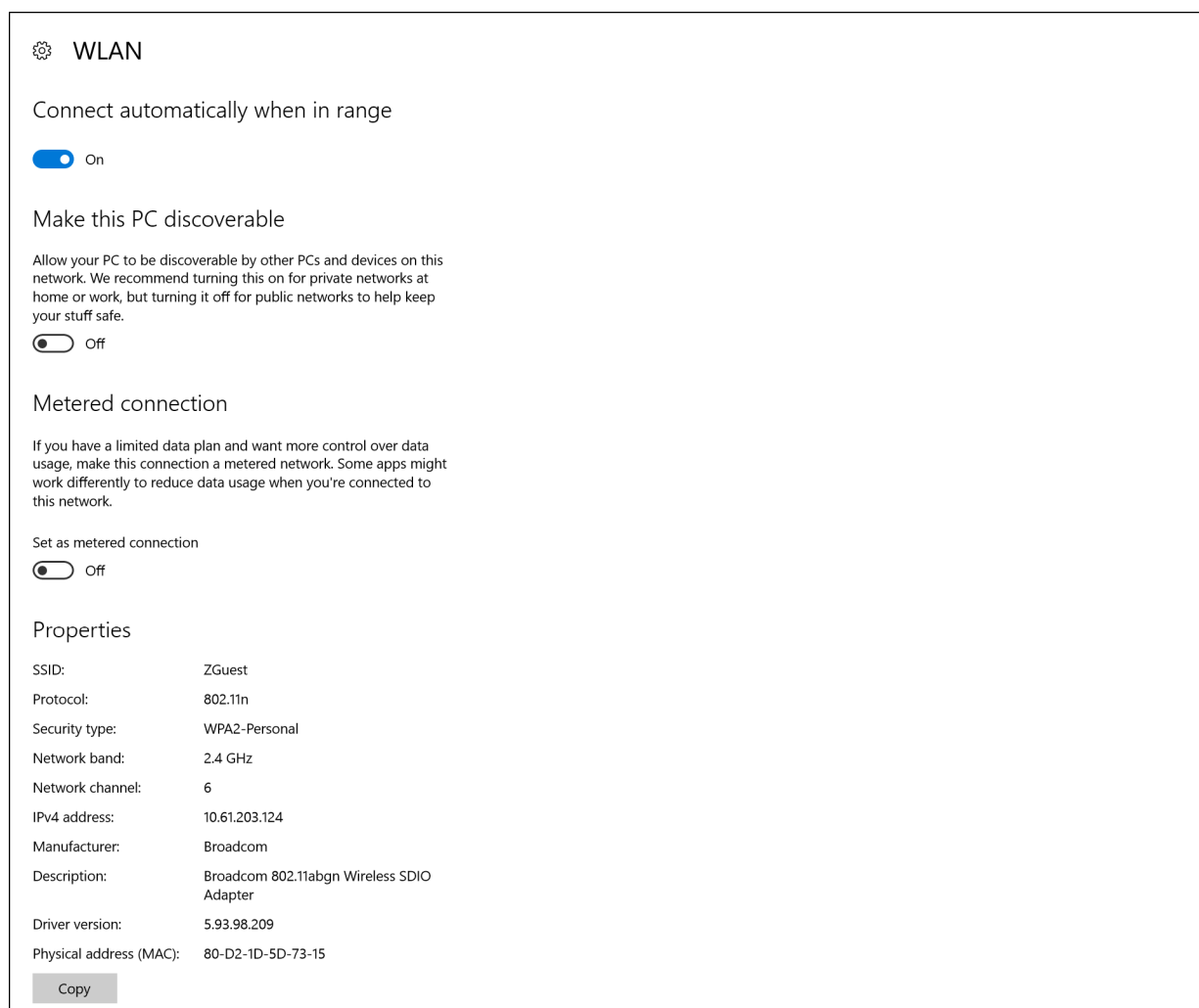
Figure 3-3 Network Information
